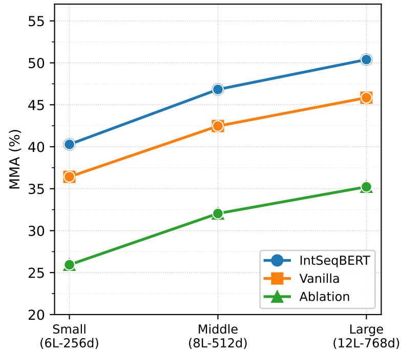
Fig. 3 Scaling Behaviour: Small \rightarrow Middle \rightarrow Large Mean Modulo Accuracy (MMA)
