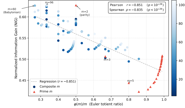
Fig. 6. NIG vs. Euler's totient ratio \phi(m)/m (Large IntSeqBERT). Composite moduli (blue circles, shade proportional to m ) and prime moduli (red triangles) are shown separately. The regression line (grey dashed) indicates Pearson r = -0.851 ( p < 10^{-28} ). Notable moduli m = 2 (parity), m = 60 (Babylonian number), and m = 96 (highly composite) are annotated.
