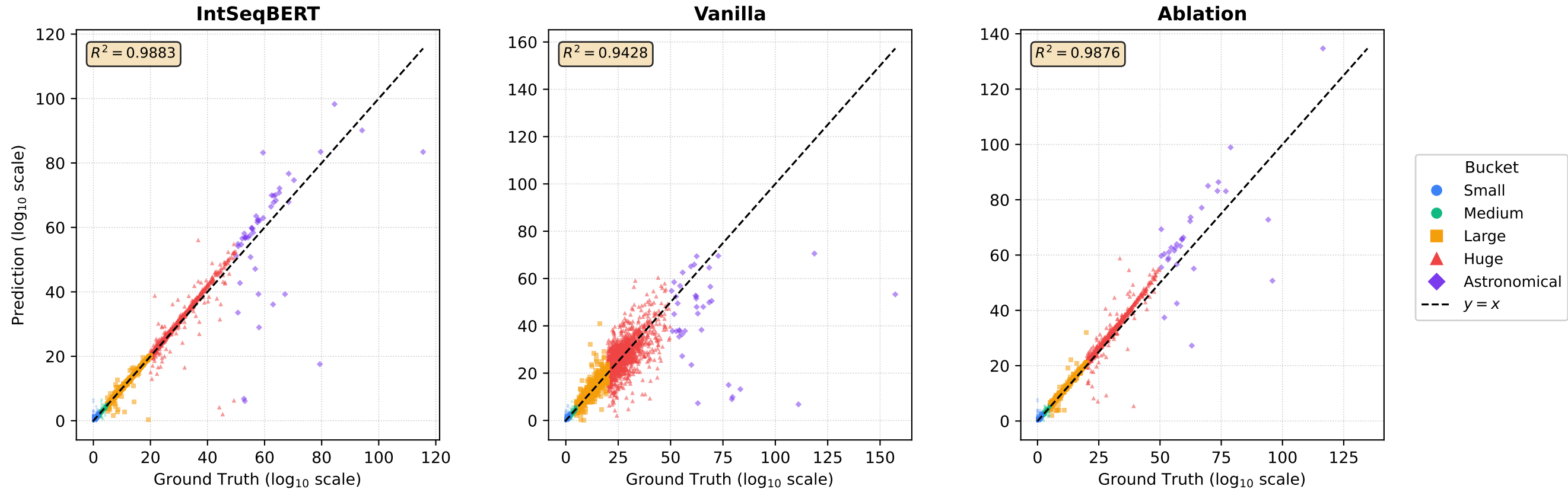
Fig. 5 Predicted vs. True Magnitude (Large models, \log_{10} scale)
