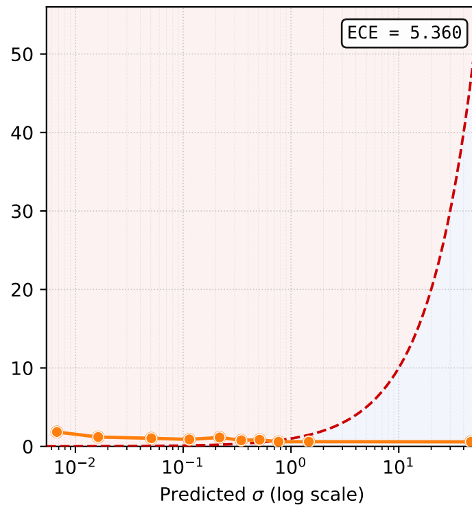
Fig. 6 Uncertainty Calibration: Predicted \sigma vs. Actual RMSE (Large models)
