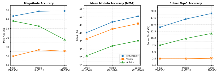
Fig. 7. Scaling behaviour (Small / Middle / Large). Left: Mag Acc improves only +1.1 pt. Centre: MMA for IntSeqBERT improves +10.1 pt (40.3% \rightarrow 50.4%). Right: Solver Top-1 improves +5.0 pt, with a growing gap over Vanilla.
