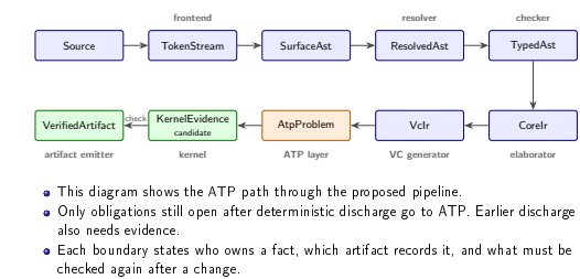
10.1 - The Core ATP Path
