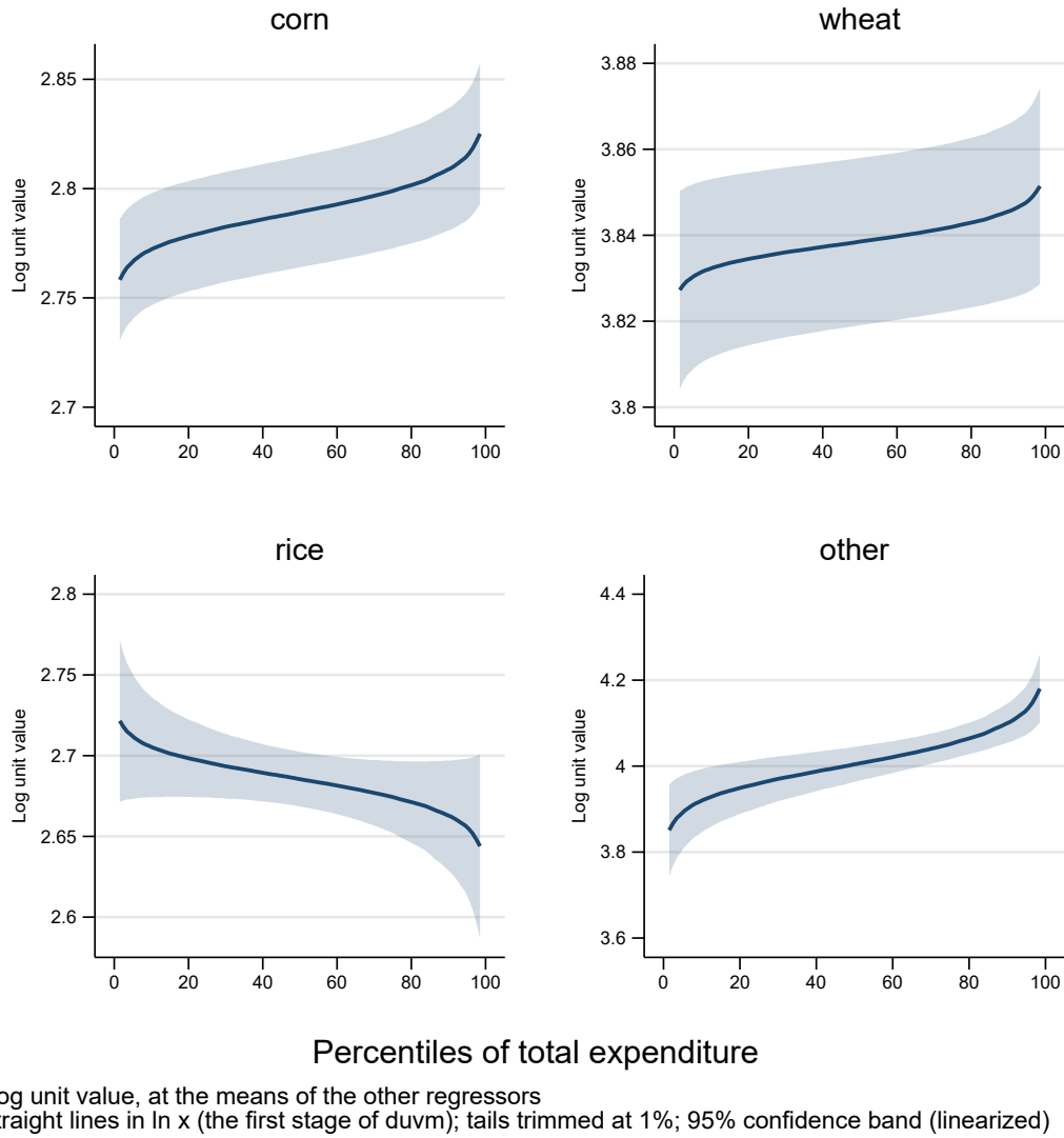
Figure 2: Engel curves of the log unit values (quality), at the means of the other regressors; 95% linearized confidence bands
