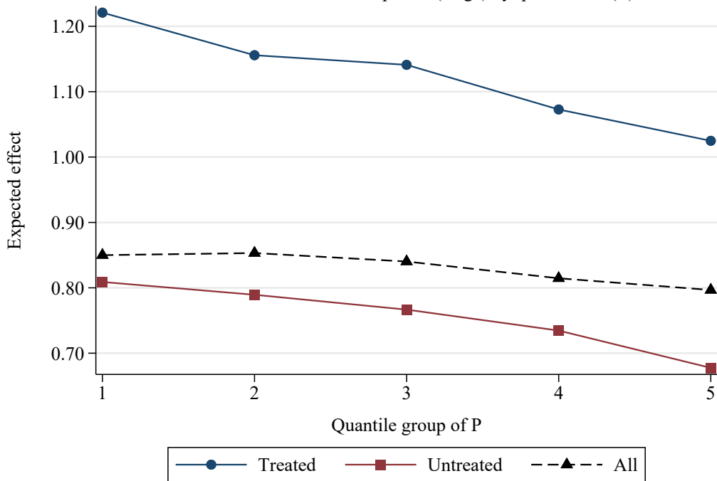
Effect of union membership on \ln(\text{wage}) by quintile of P(Z)
