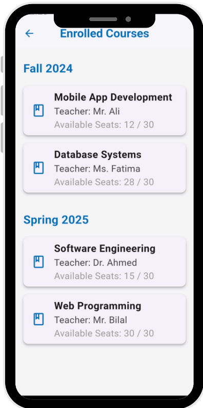
Enrolled Courses
