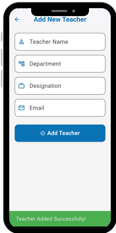
Add Teacher
