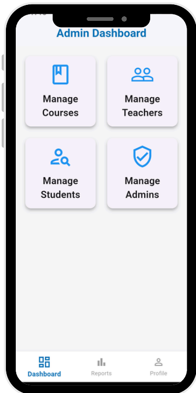
Admin Dashboard
