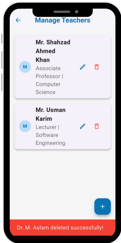
Manage Teacher
