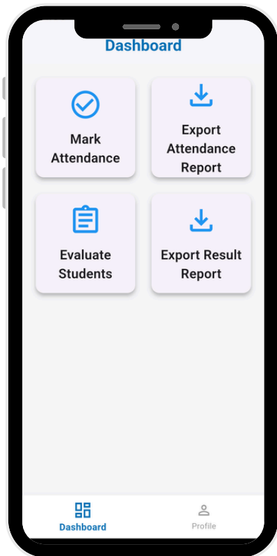
Teacher Dashboard
