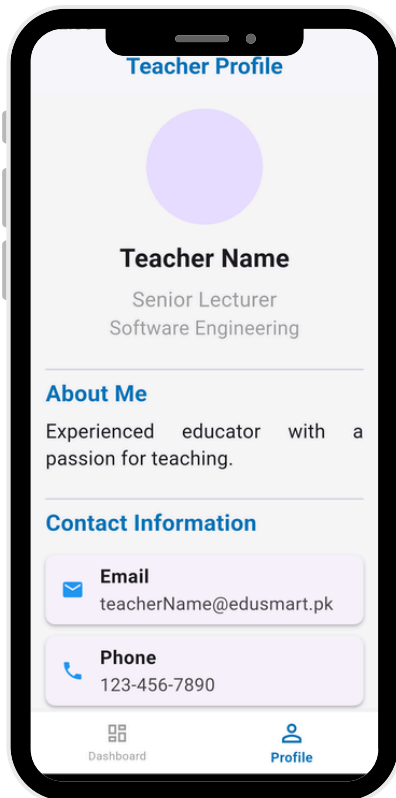
Teacher Profile
