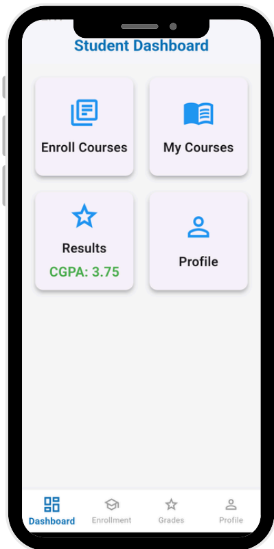
Student Dashboard
