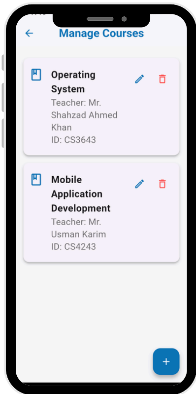
Manage Courses
