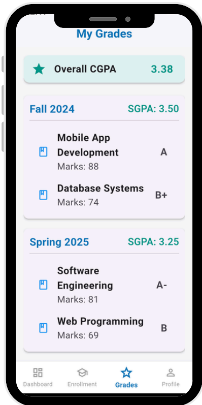
Student Result
