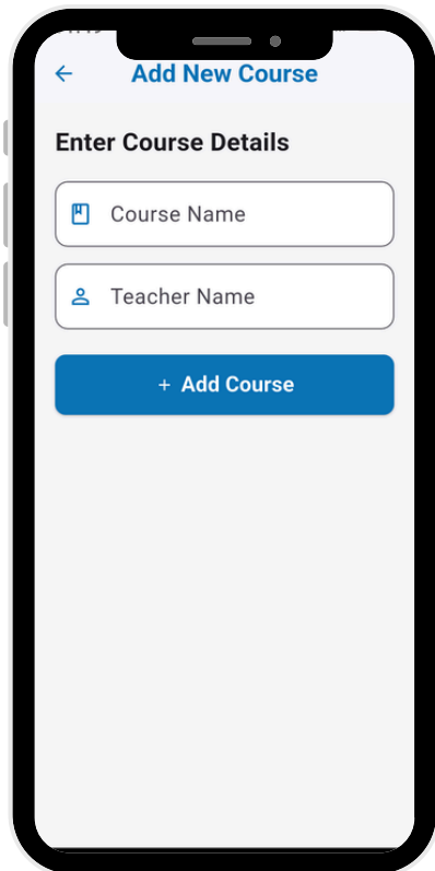
Add Courses
