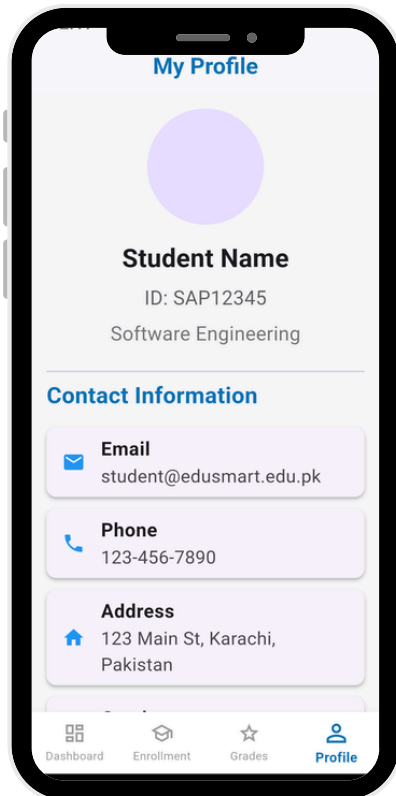
Student Profile
