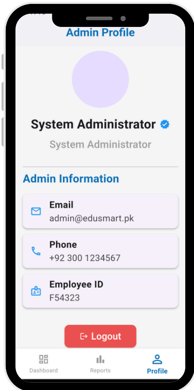
Admin Profile
