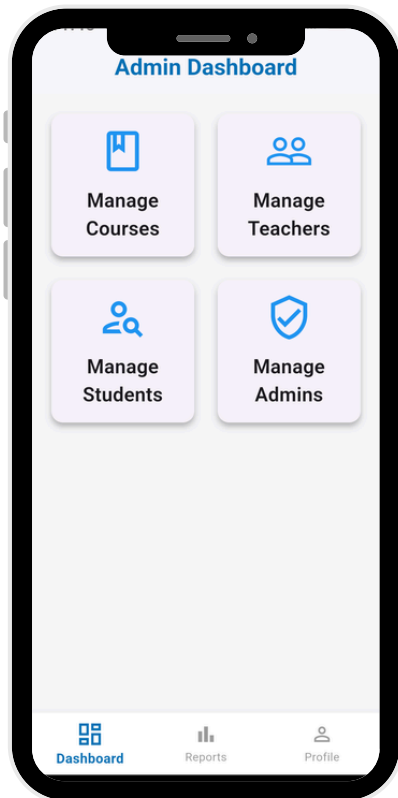
Admin Dashboard
