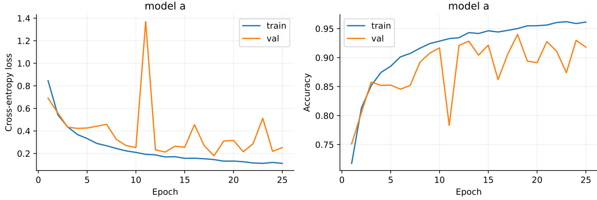
Figure 2: Model A training and validation history.
