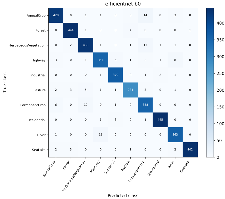
Figure 9: EfficientNet-B0 test confusion matrix (counts).
