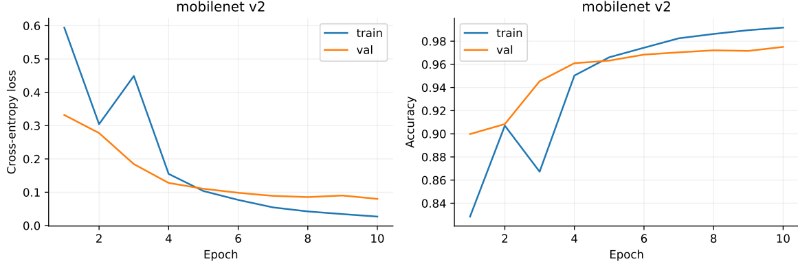
Figure 6: MobileNetV2: frozen-head epochs 1–2 and full-network fine-tuning epochs 3–10.
