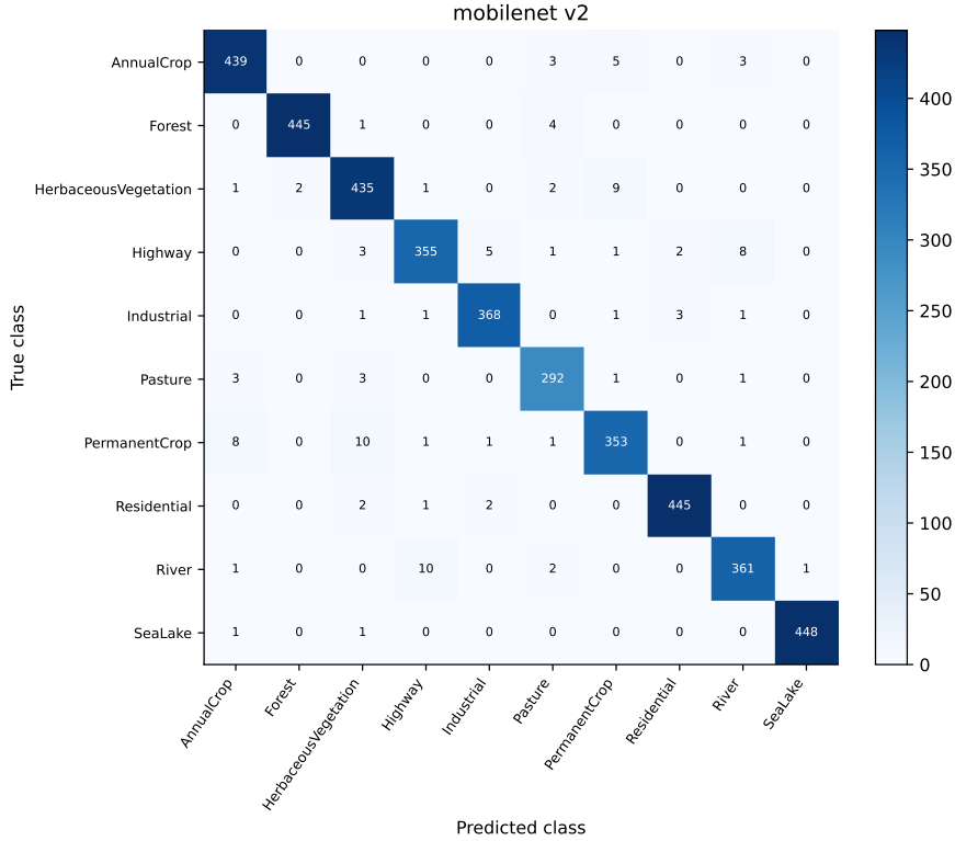
Figure 7: MobileNetV2 test confusion matrix (counts).
