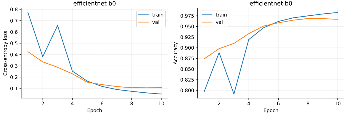
Figure 8: EfficientNet-B0: frozen-head epochs 1–2 and full-network fine-tuning epochs 3–10.
