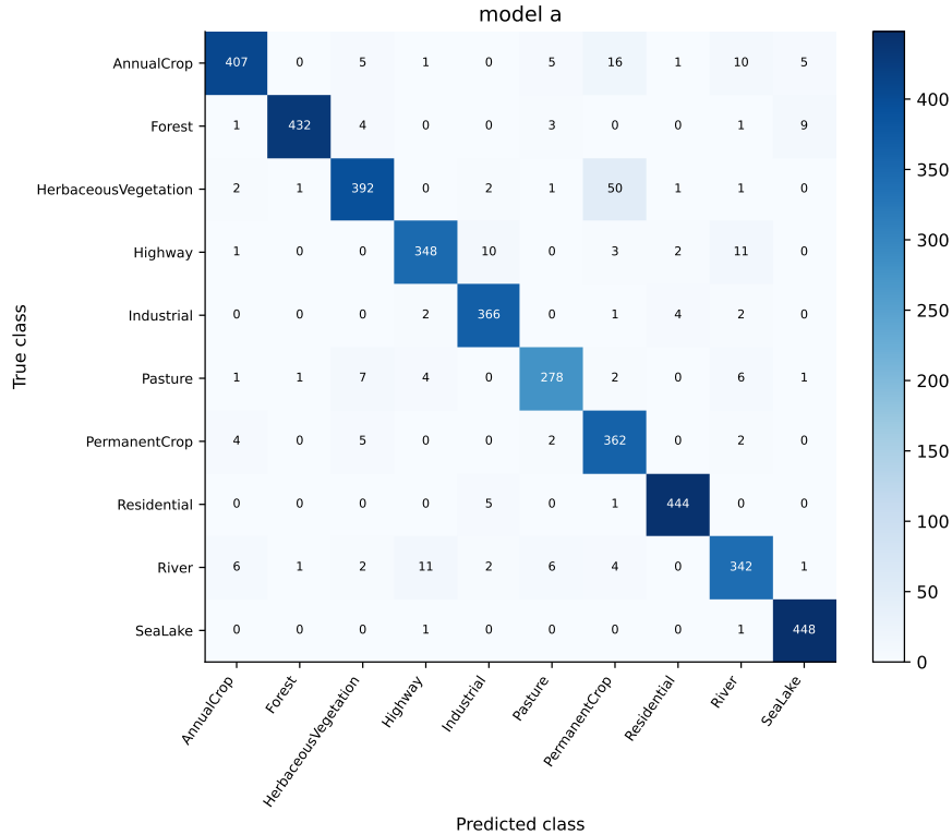
Figure 4: Model A: numeric counts, true classes on rows and predictions on columns.
