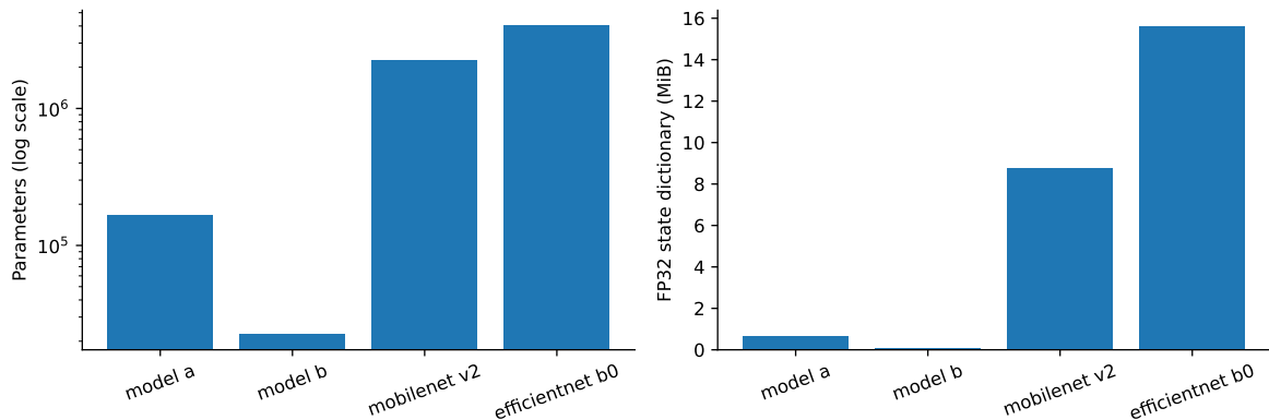
Figure 11: Parameter counts and measured FP32 state-dictionary sizes.
