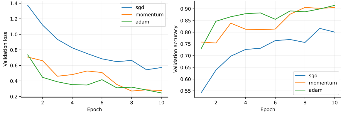
Figure 1: Validation loss and accuracy; unsmoothed observations.
