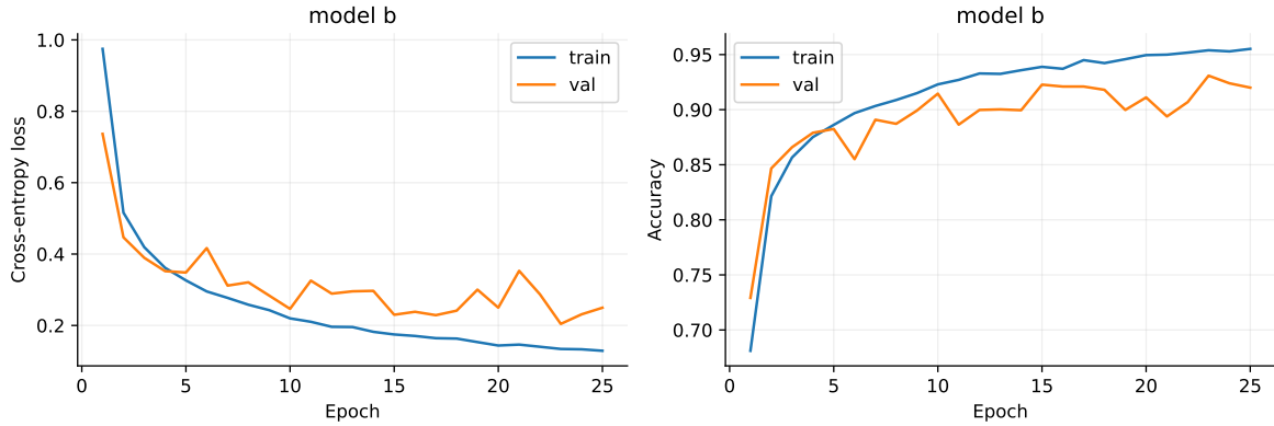
Figure 3: Model B training and validation history.
