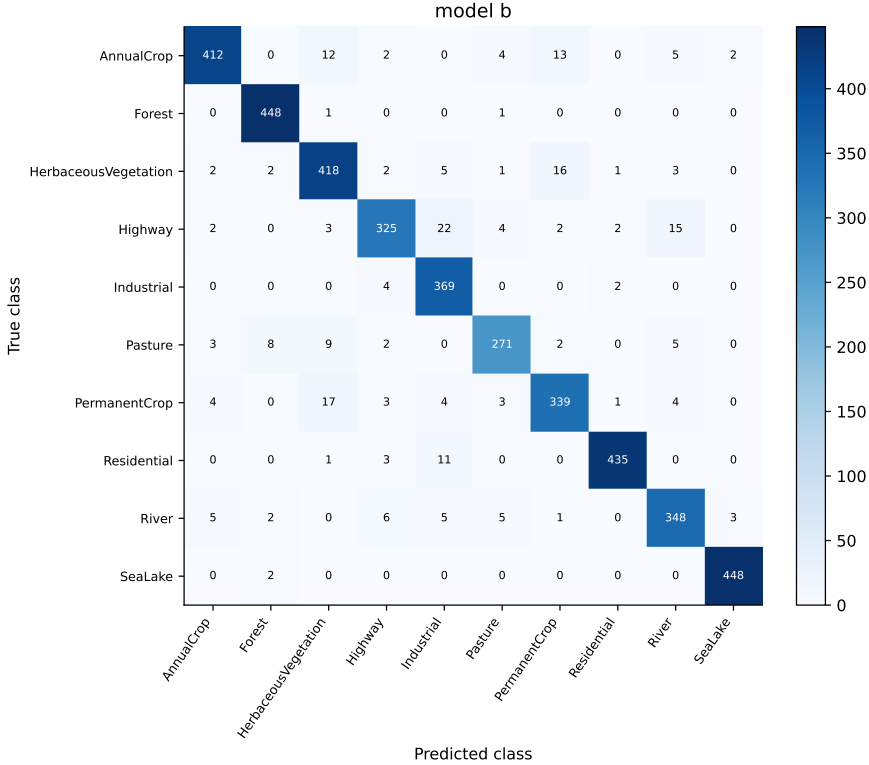
Figure 5: Model B: numeric counts, true classes on rows and predictions on columns.
