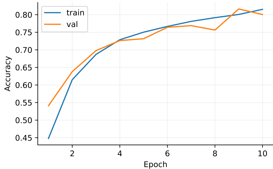
optimizer sgd
