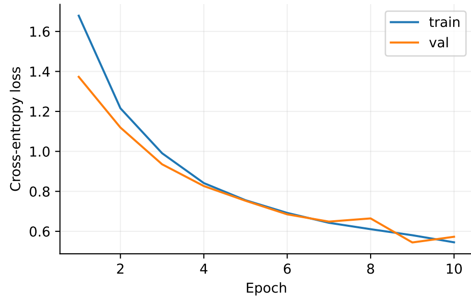
optimizer sgd
