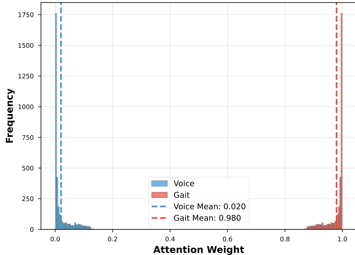
Distribution of Attention Weights
