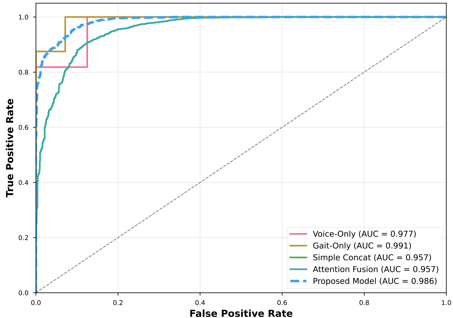
ROC Curves: Parkinson's Disease Detection
