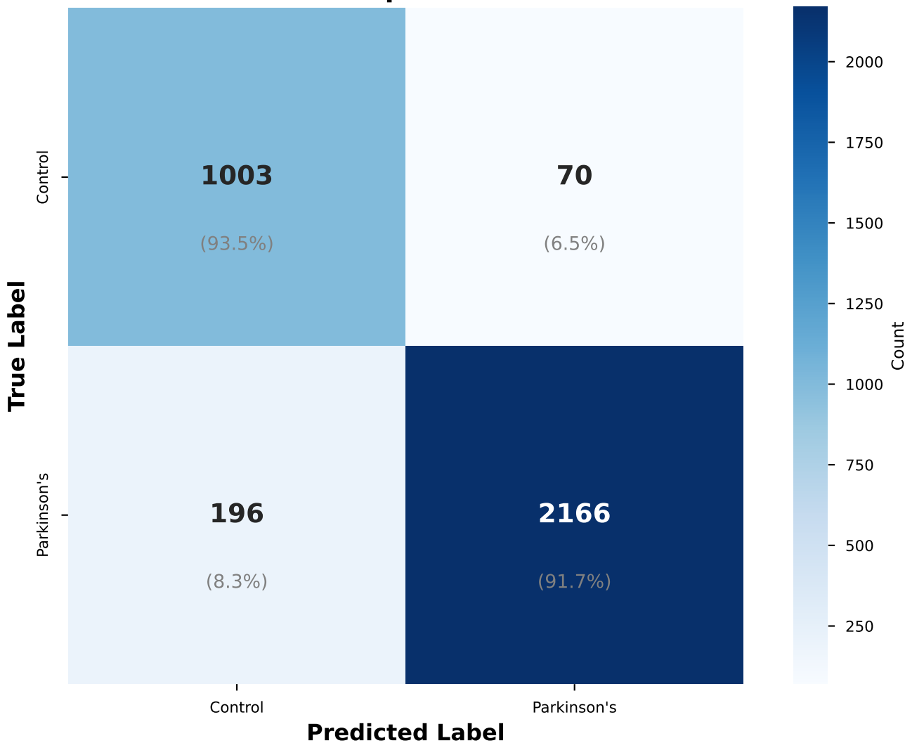
Confusion Matrix: Proposed Multimodal Model
