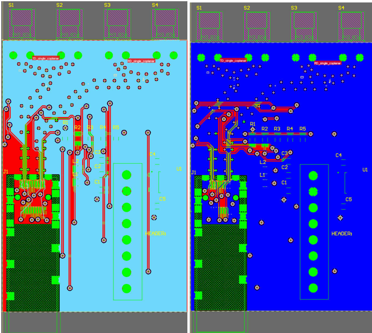
Figure 2: Inner layer 2 and Bottom layer
