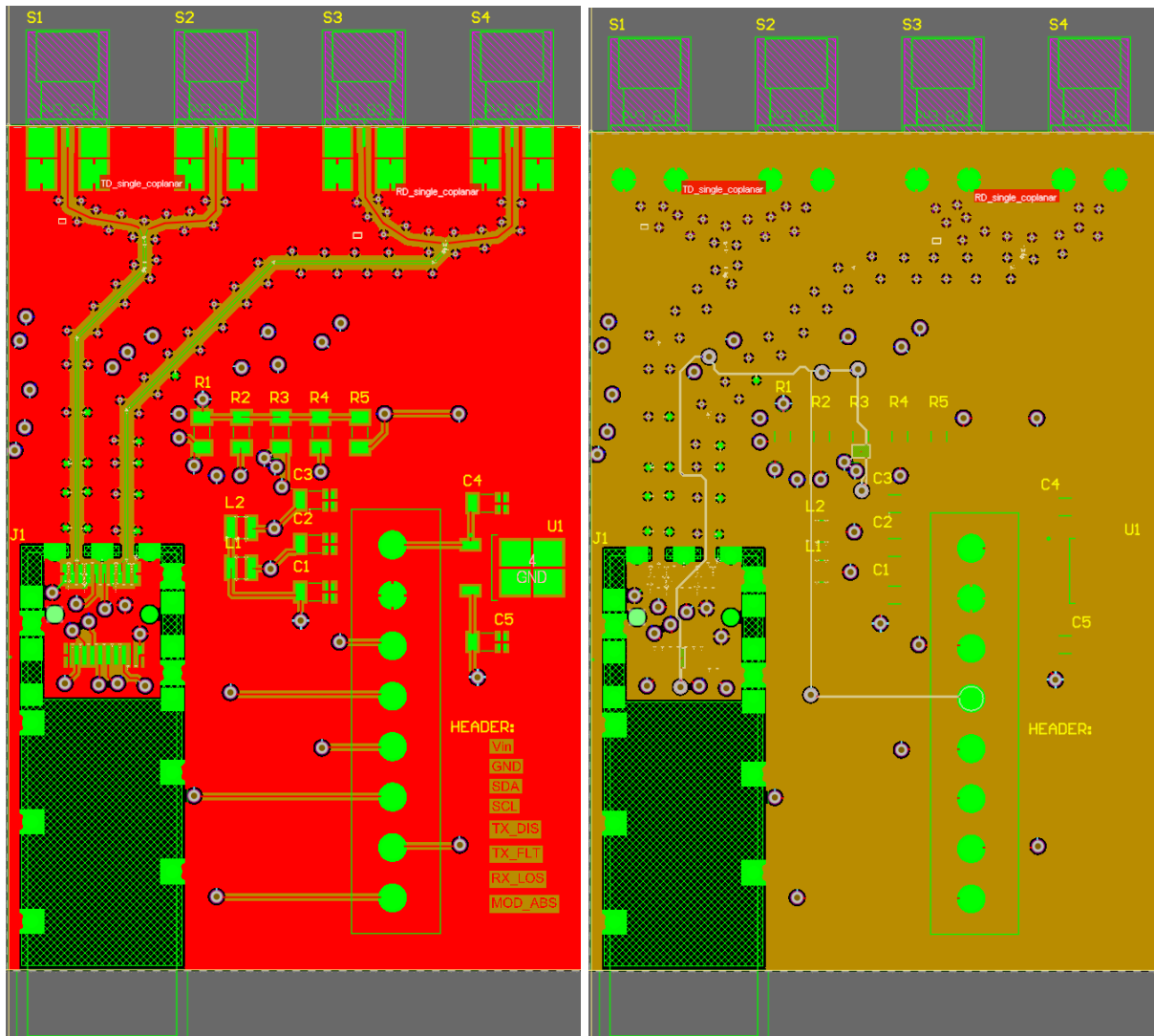
Figure 1: Top layer and Inner Layer 1
