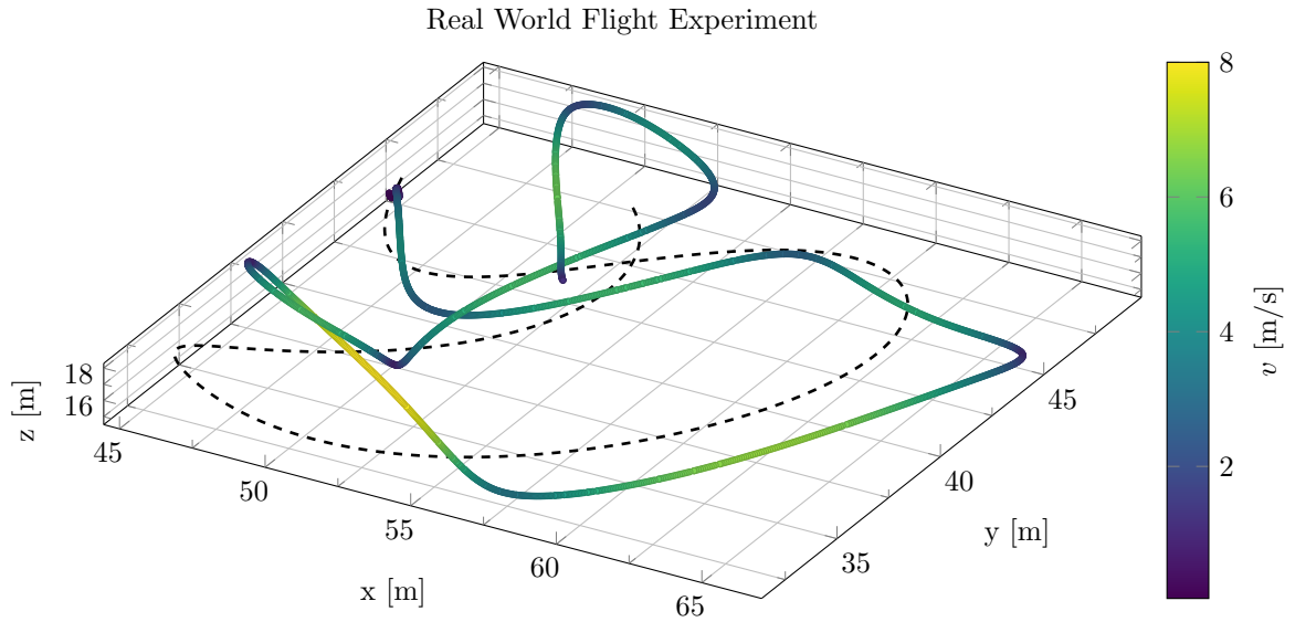
Figure 4.8: Real world flight data, UZH track trajectory tracking.
