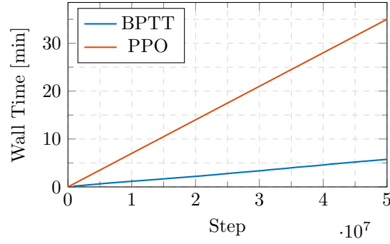
Figure 4.4: Wall time versus training steps for PPO and BPTT.
