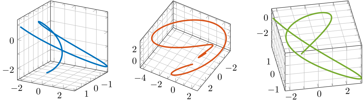
Figure 3.6: Training trajectories generated from the sum of harmonics.
