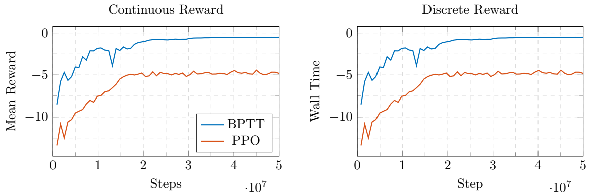
Figure 4.5: Comparison between BPTT and PPO when the loss is countinuous or discrete.
