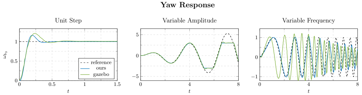
Figure 4.3: Yaw response to unit step, variable amplitude and variable frequency signals.
