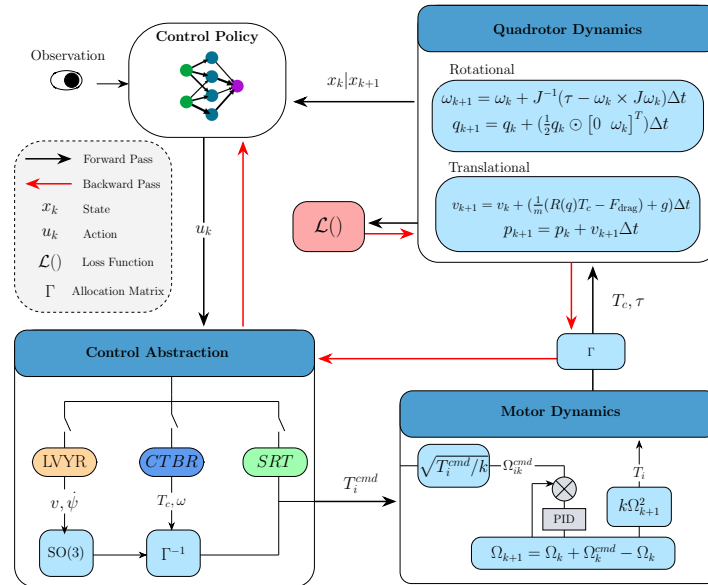
Figure 3.1: Schematics of the learning environment. The black arrows show the forward pass from the policy outputs to the loss function and the red arrows indicate the backward pass. Not that during the backward pass the motor dynamics are skipped.
