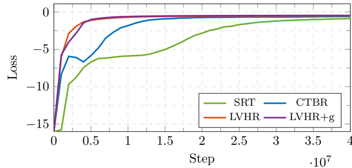
Figure 4.7: Loss versus time step for the different control abstractions.
