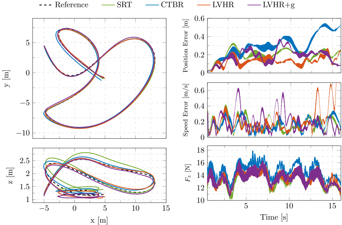
Figure 4.8: Tracking error of the different control abstractions for the UZH racing track.
