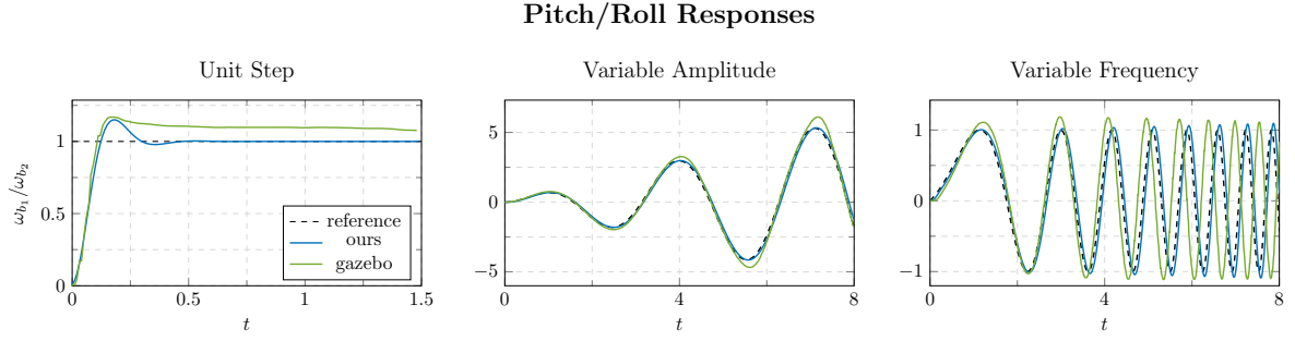
Figure 4.2: Pitch/Roll responses to unit step, variable amplitude and variable frequency signals.
