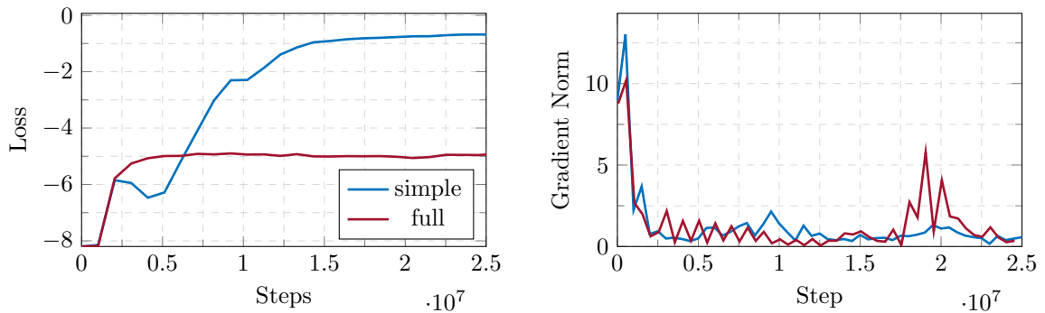
Figure 4.8: Gradients.
