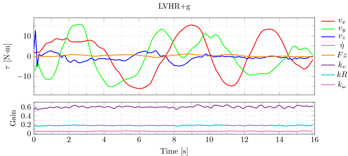
Figure 4.9: Linear velocities, heading rate and controller gains commands for the UZH trajectory.
