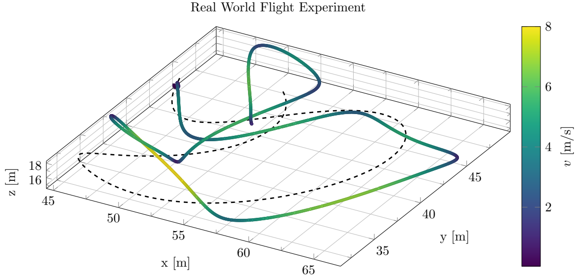
Figure 4.11: Real world trajectory.
