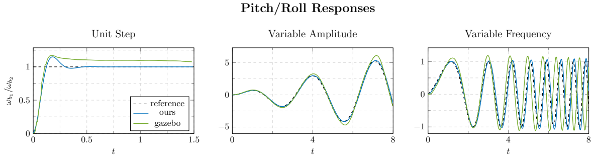
Figure 4.2: Pitch/Roll responses to unit step, variable amplitude and variable frequency signals.
