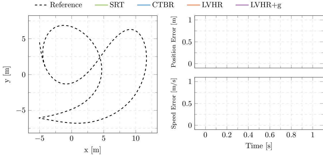
Figure 4.8: Tracking error of the different control abstractions for the UZH racing track.
