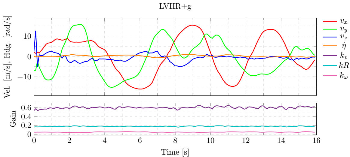
Figure 4.9: Commanded linear velocities, heading rate and controller gains for the UZH trajectory.
