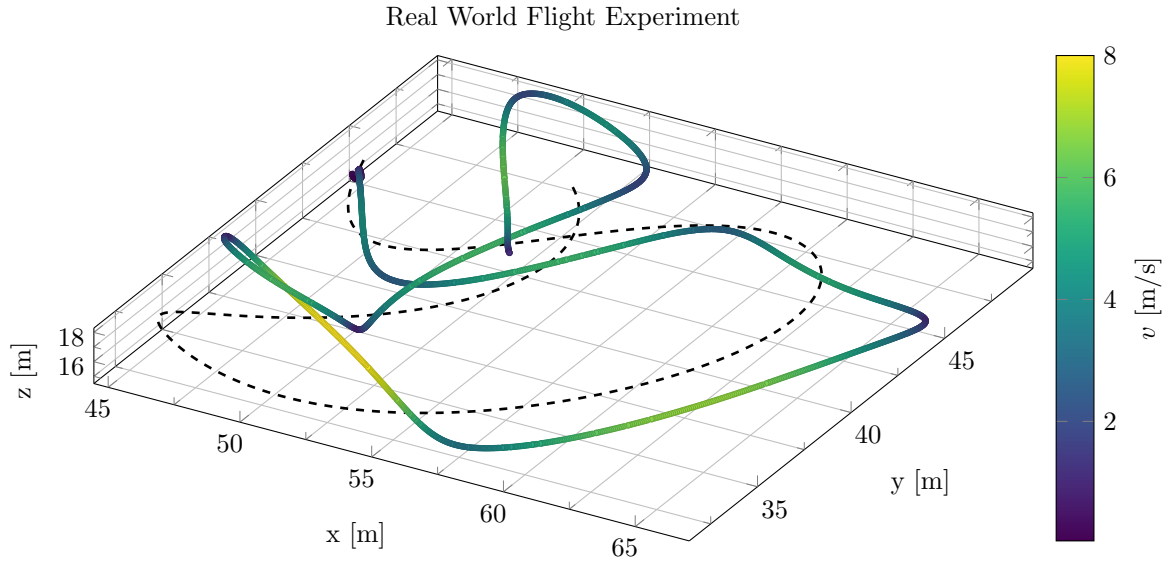
Figure 4.11: Real world flight data, UZH track trajectory tracking.
