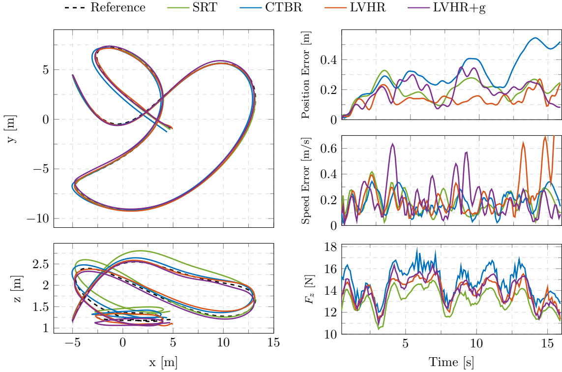
Figure 4.5: Tracking error of the different control abstractions for the UZH racing track.
