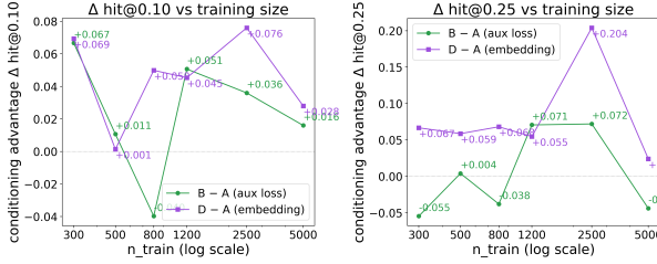
Figure 4. Exploratory conditioning advantage ( \Delta \text{hit@0.10} vs. A) across n_{\text{train}} . Caveat from Section 5.2: each historical size used a different val slice with different goal leakage (up to 85%), so this curve is directional at best; the confirmatory grid (Table 7) fixes one frozen test set for all sizes.
