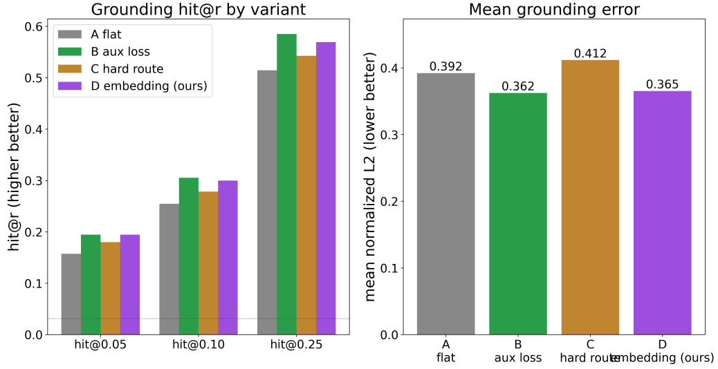
Figure 3: Exploratory ablation on all_with_coords (historical splits; per-seed values). Shown for continuity with the historical record; Table 6 carries the calibrated statistics and Table 1 the confirmatory test-set versions.
