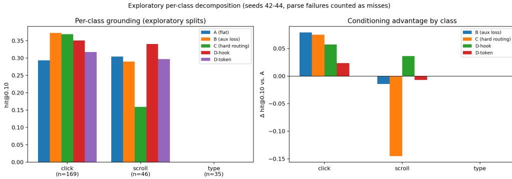
Figure 2: Exploratory hit@0.10 by action class ( all_with_coords ). The conditioning advantage concentrates in click ; type is degenerate on AITW (all variants score exactly 0.000, mean L2 at the \approx \sqrt{2} corner-to-corner distance).
