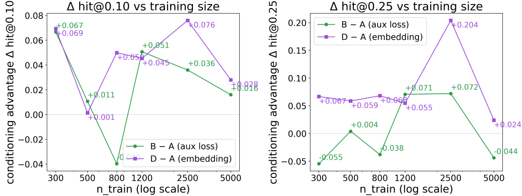
Figure 4: Exploratory conditioning advantage ( \Delta \text{hit}@0.10 vs. A) across n_{\text{train}} . Caveat from Section 5.2: each historical size used a different val slice with different goal leakage (up to 85%), so this curve is directional at best; the confirmatory grid (Table 4) fixes one frozen test set for all sizes.
