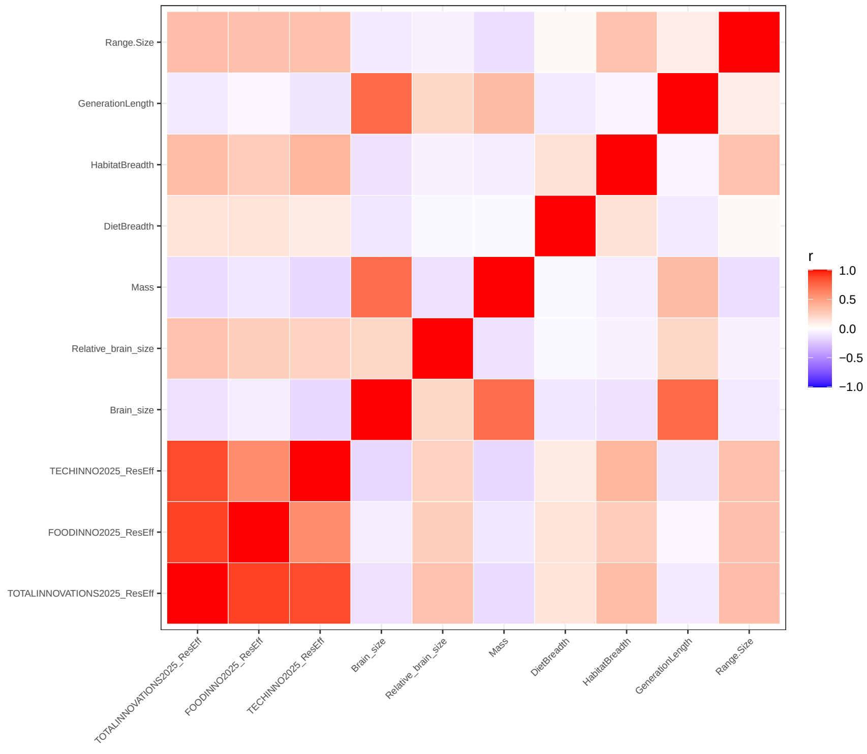
Trait correlation matrix
