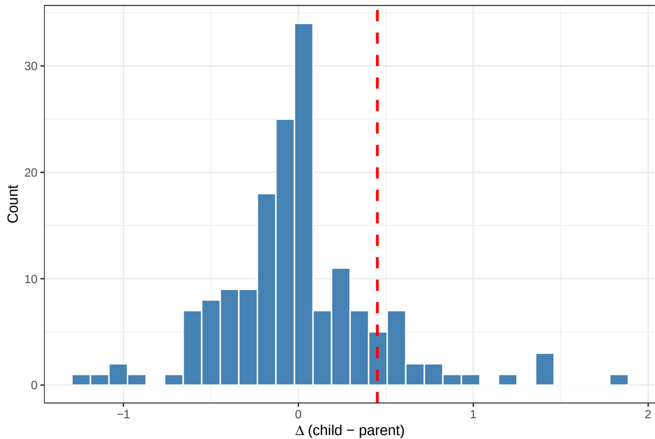
Distribution of branch-wise trait changes
