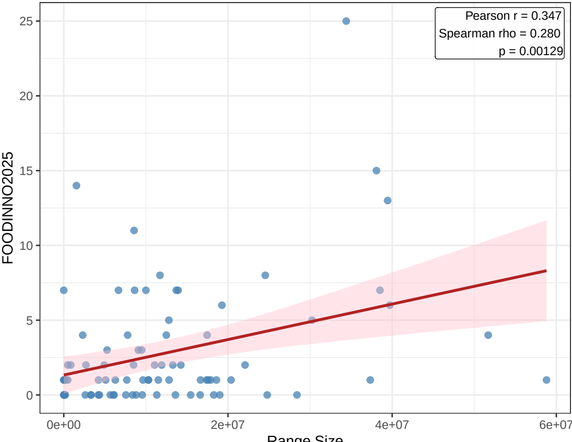
FOODINNO2025 vs Range.Size
