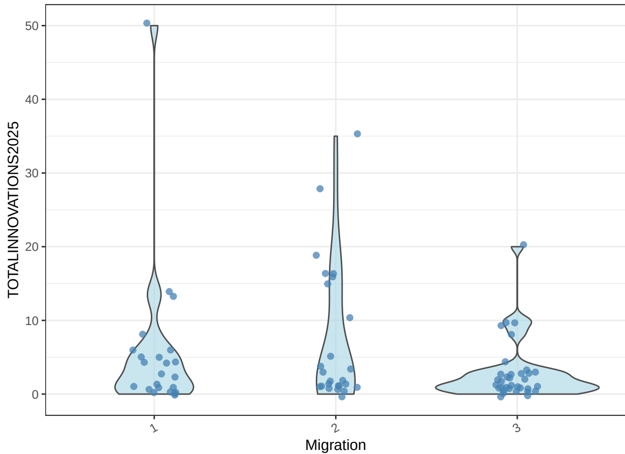
TOTALINNOVATIONS2025 by Migration (violin)
