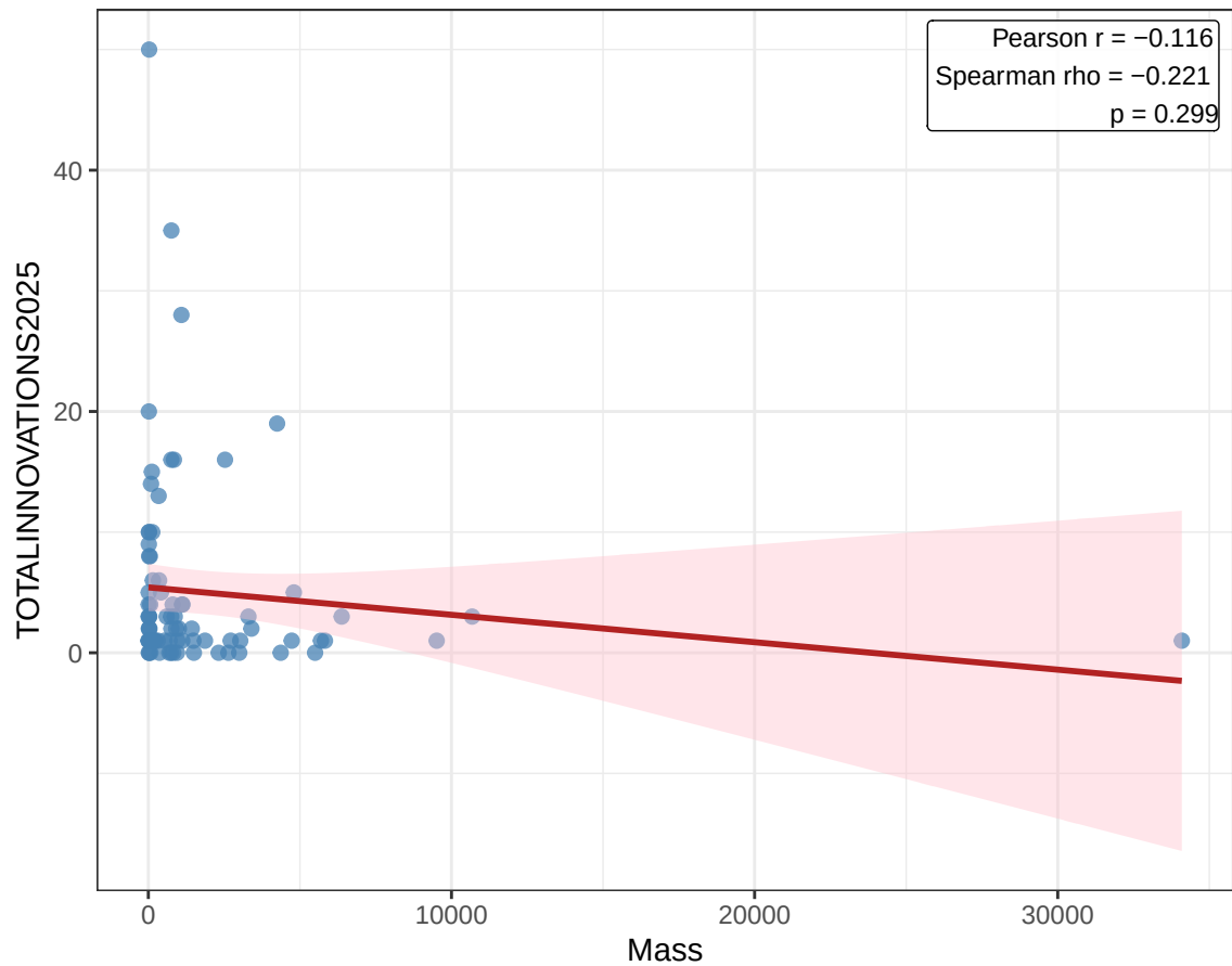
TOTALINNOVATIONS2025 vs Mass
