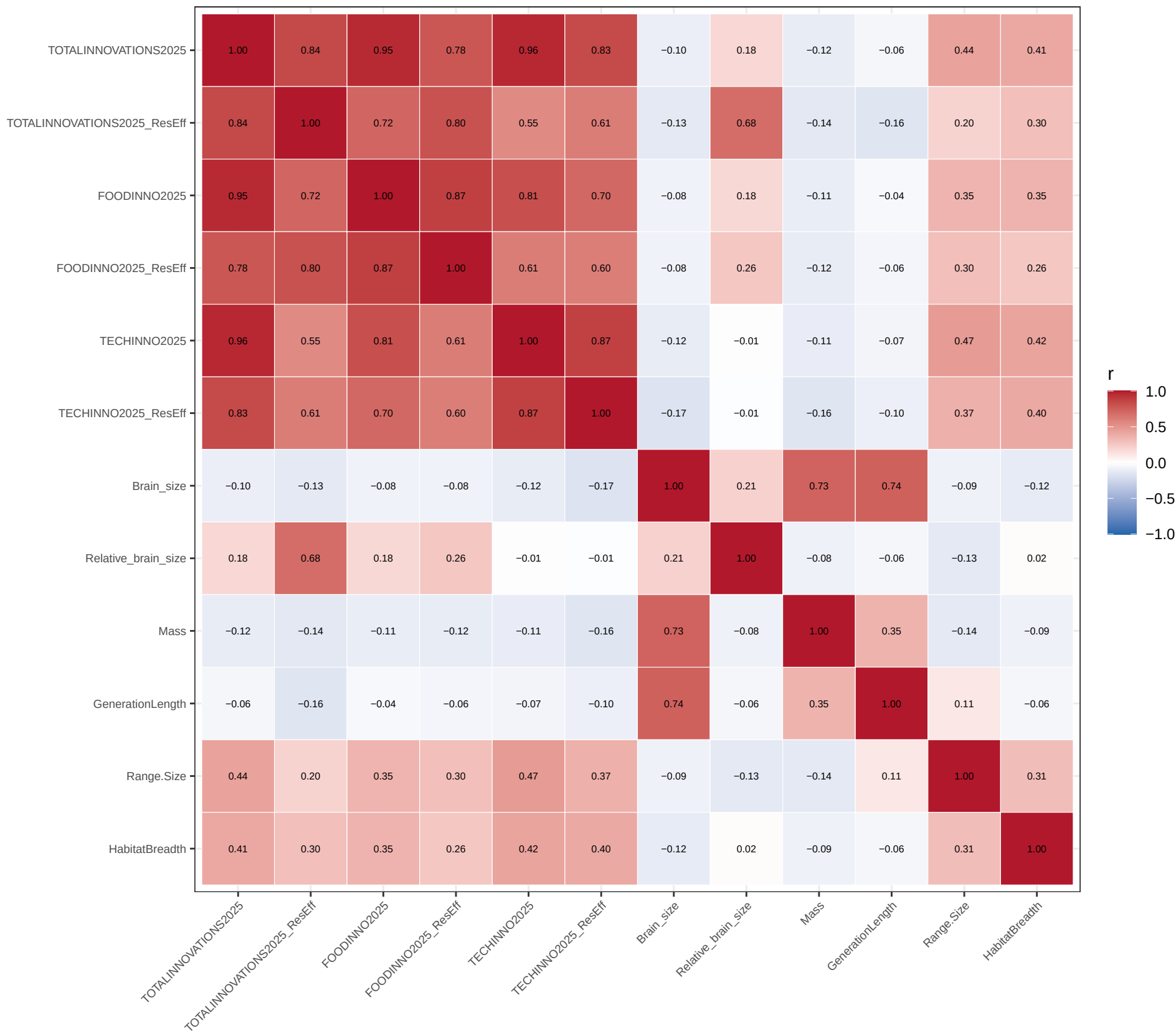
Innovation and trait correlation matrix (Pearson, pairwise complete)
