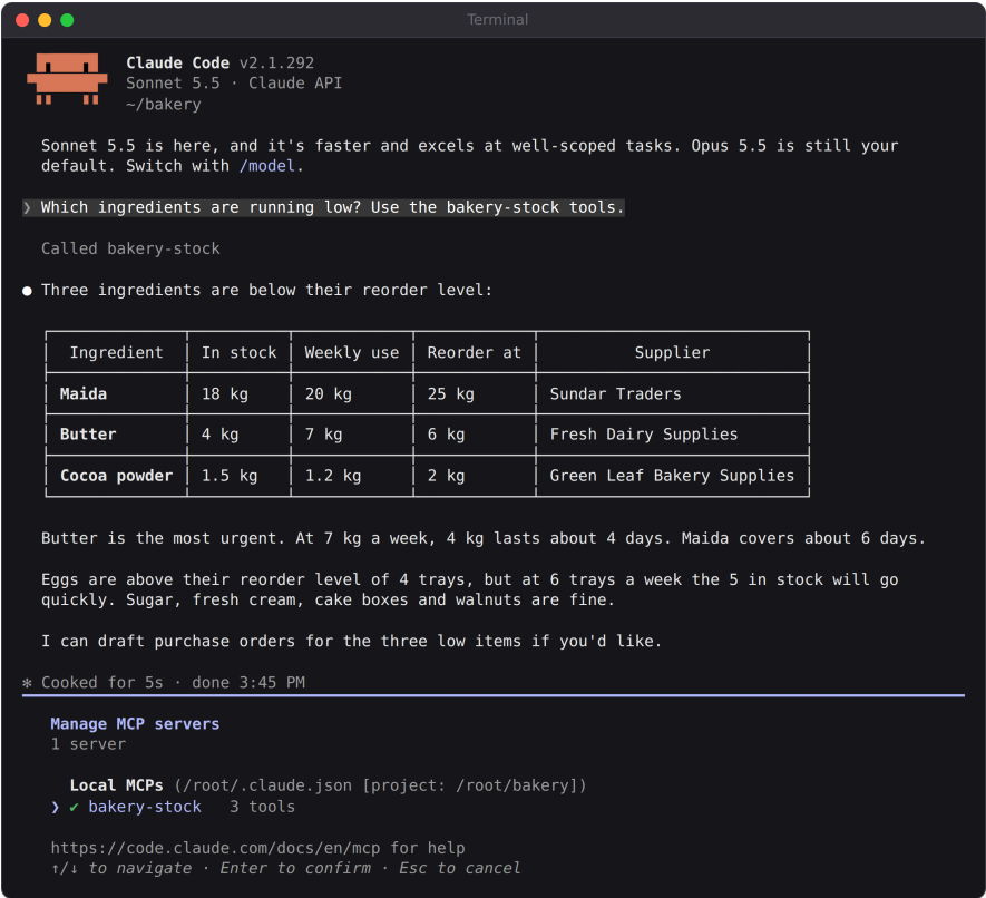
The /mcp screen in Claude Code, showing the bakery-stock server connected with 3 tools.
