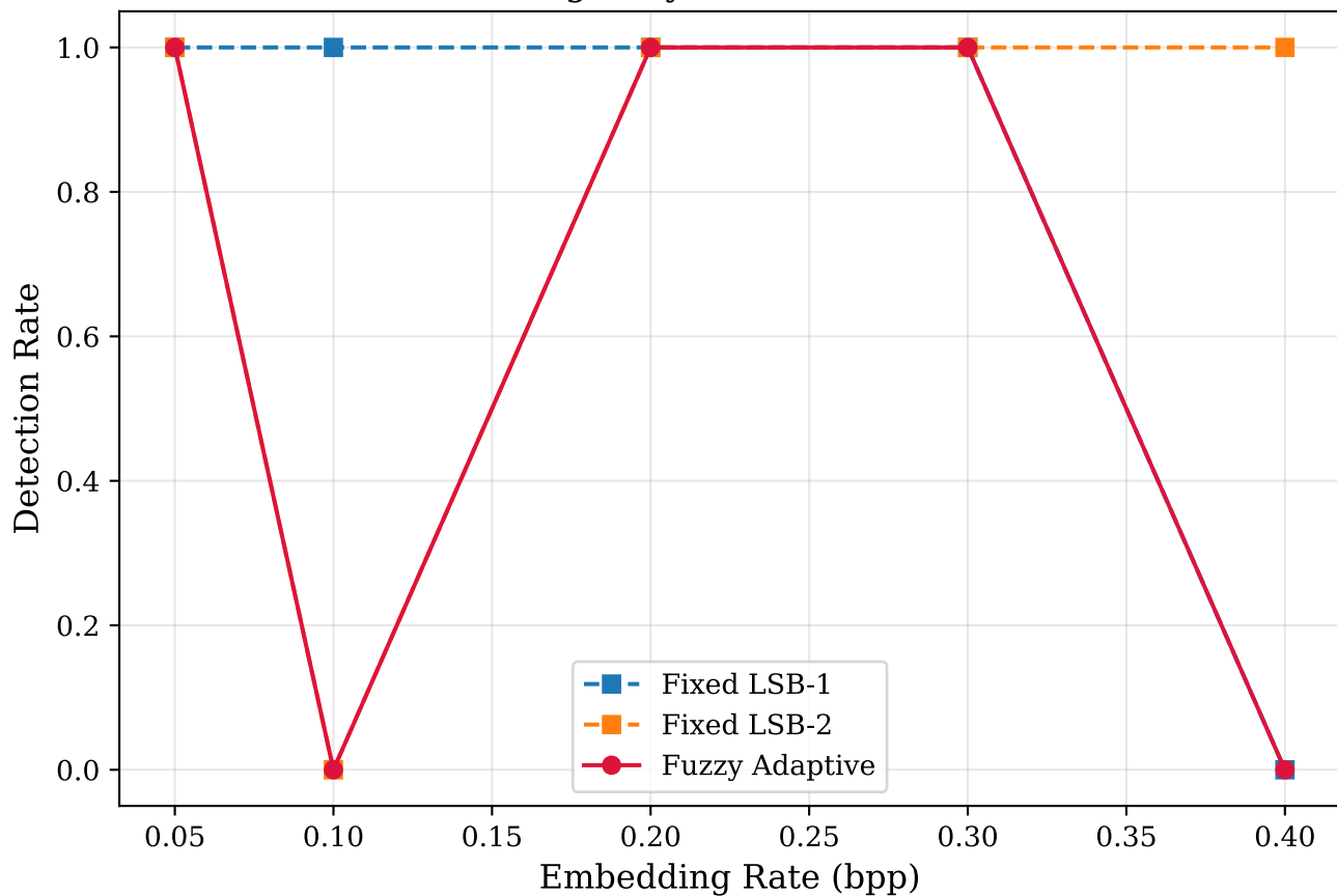
RS Steganalysis Detection Rate
