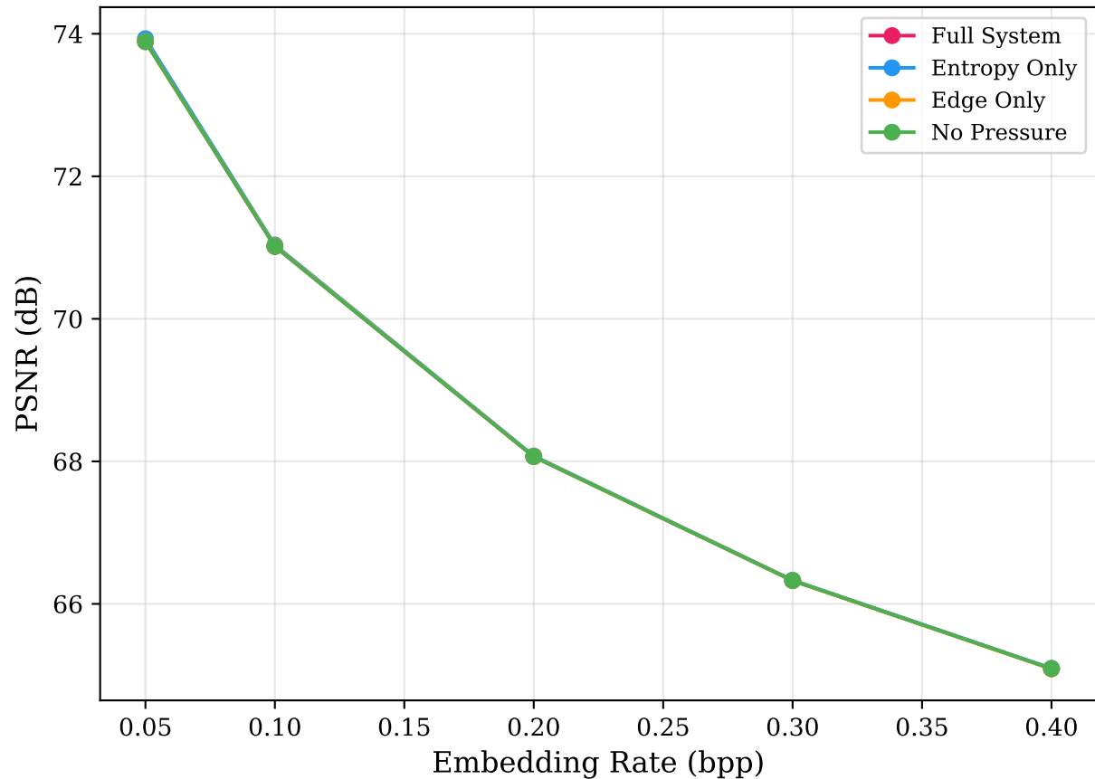
Ablation: Image Quality
