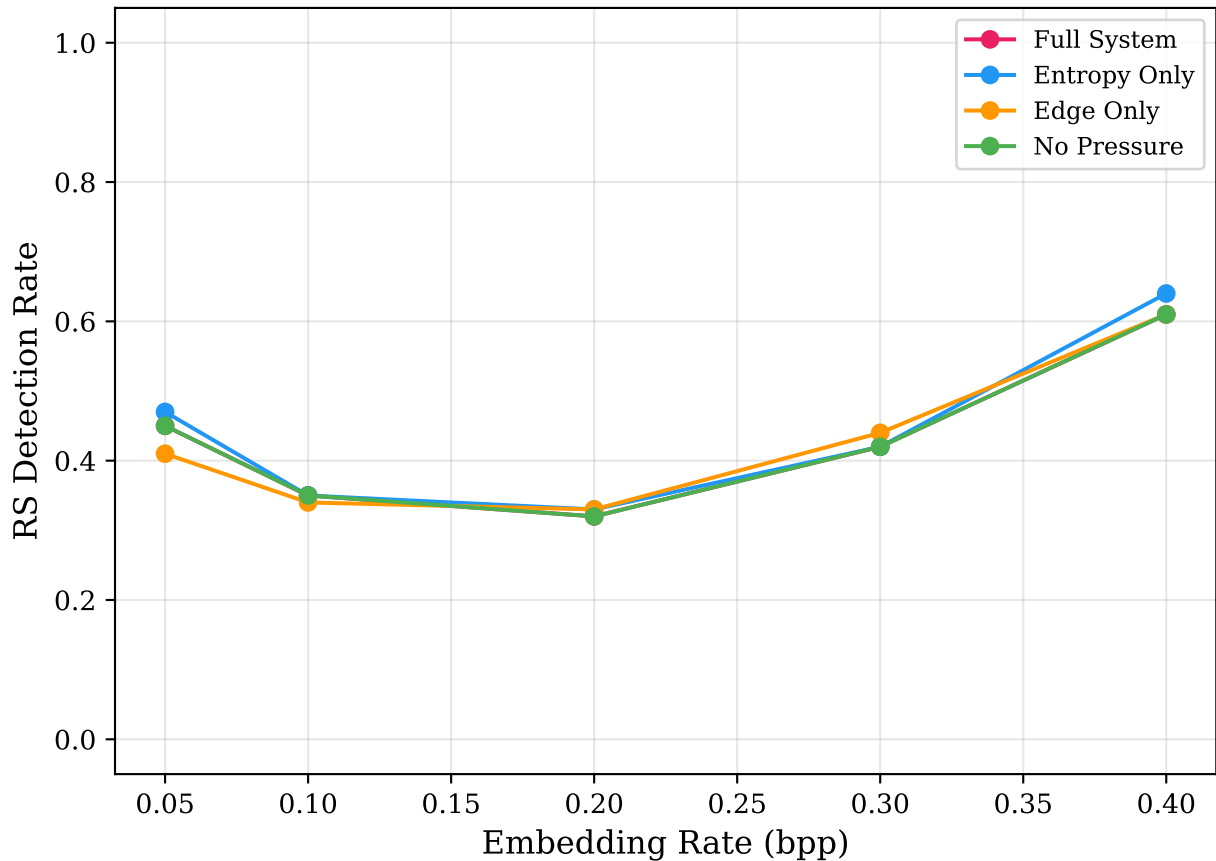
Ablation: Detection Rate
