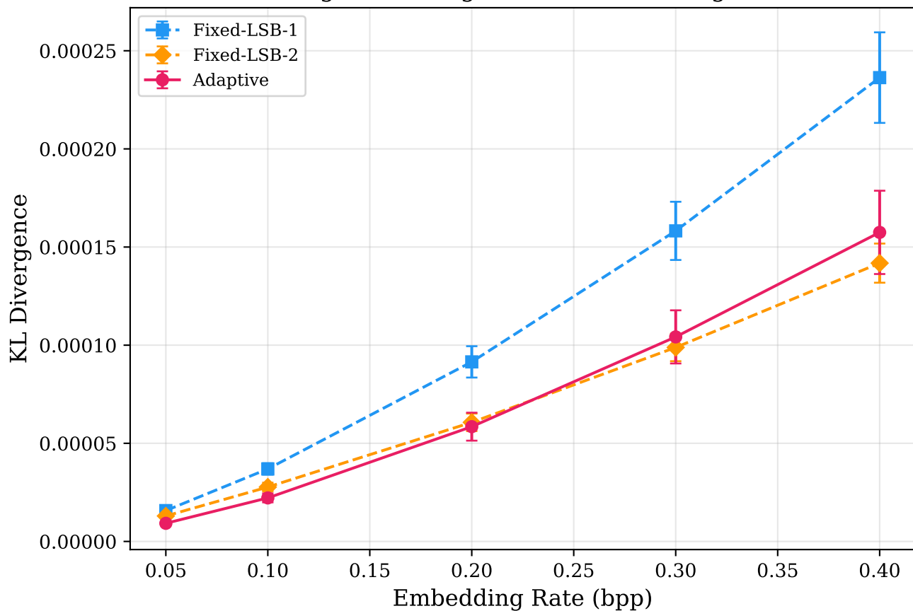
Histogram Divergence vs. Embedding Rate
