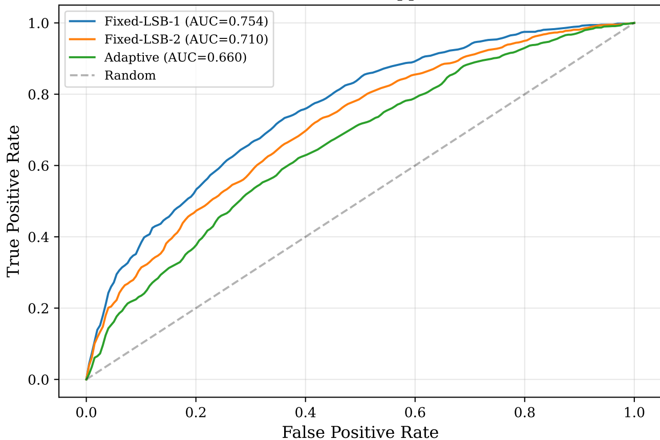
ROC Curves at bpp=0.05
