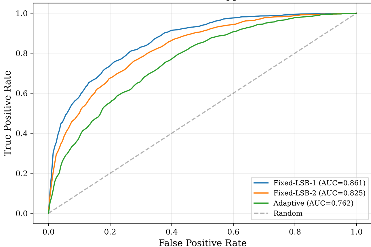
ROC Curves at bpp=0.1
