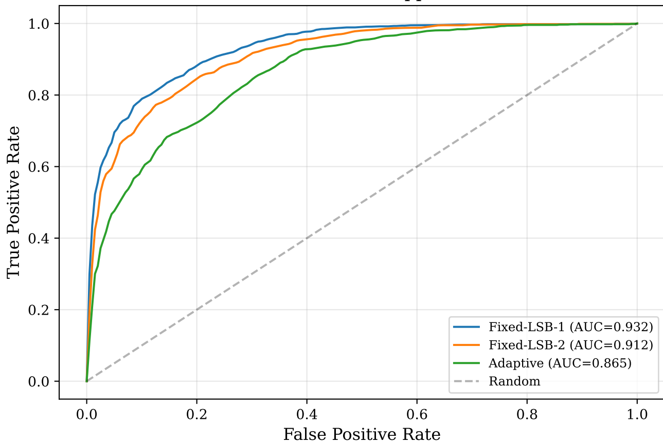
ROC Curves at bpp=0.2
