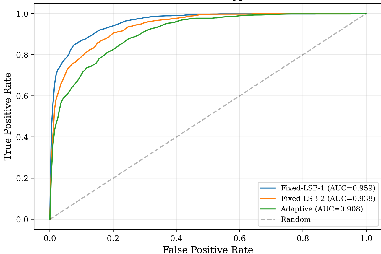
ROC Curves at bpp=0.3
