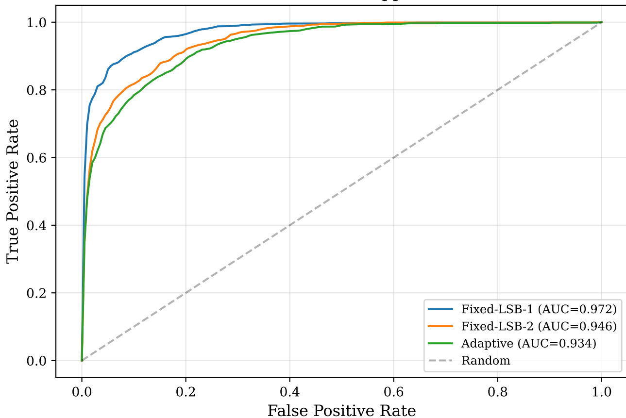
ROC Curves at bpp=0.4
