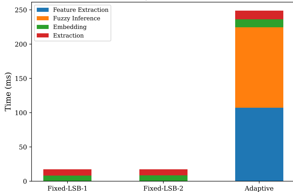
Processing Time Breakdown
