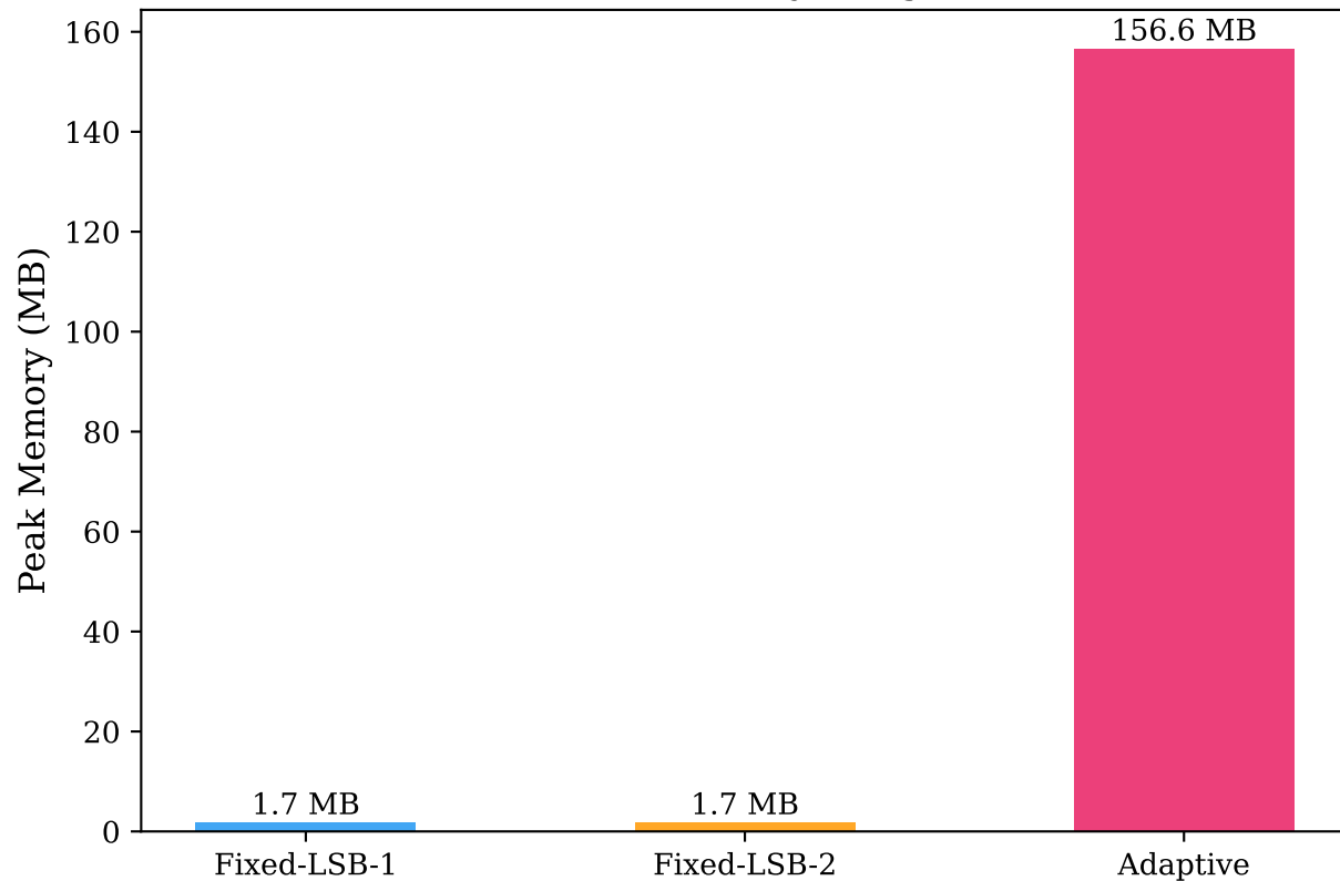
Peak Memory Usage
