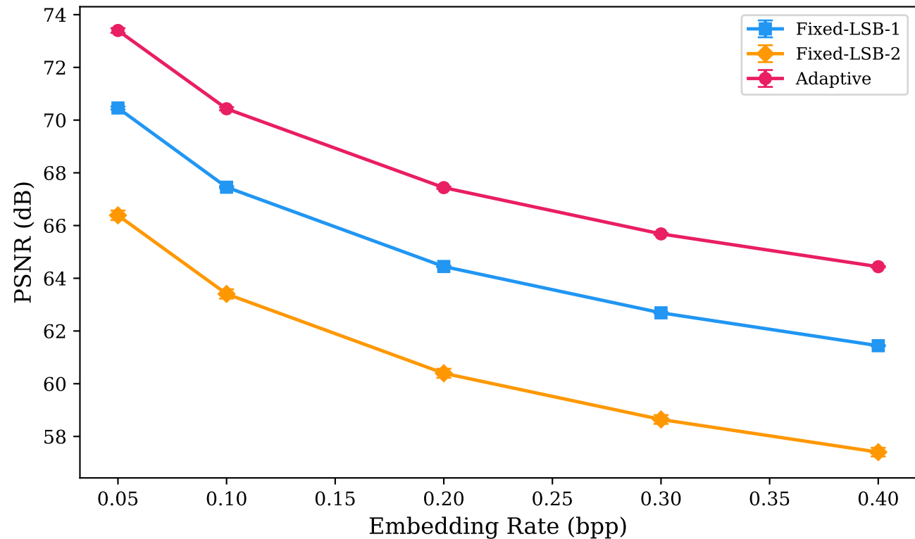
PSNR vs BPP — MIRFLICKR-25000
