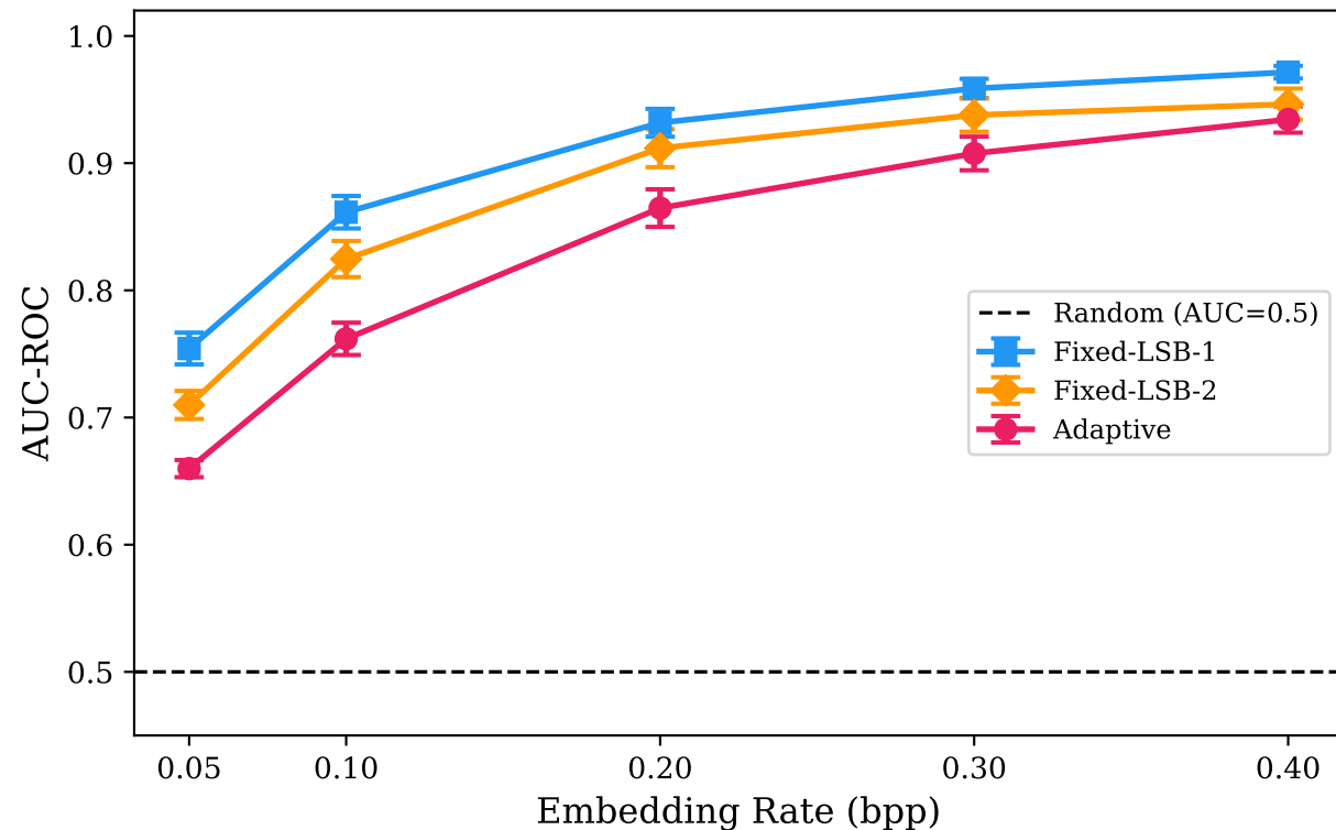
SRM-lite Detector AUC vs BPP (lower = harder to detect)
