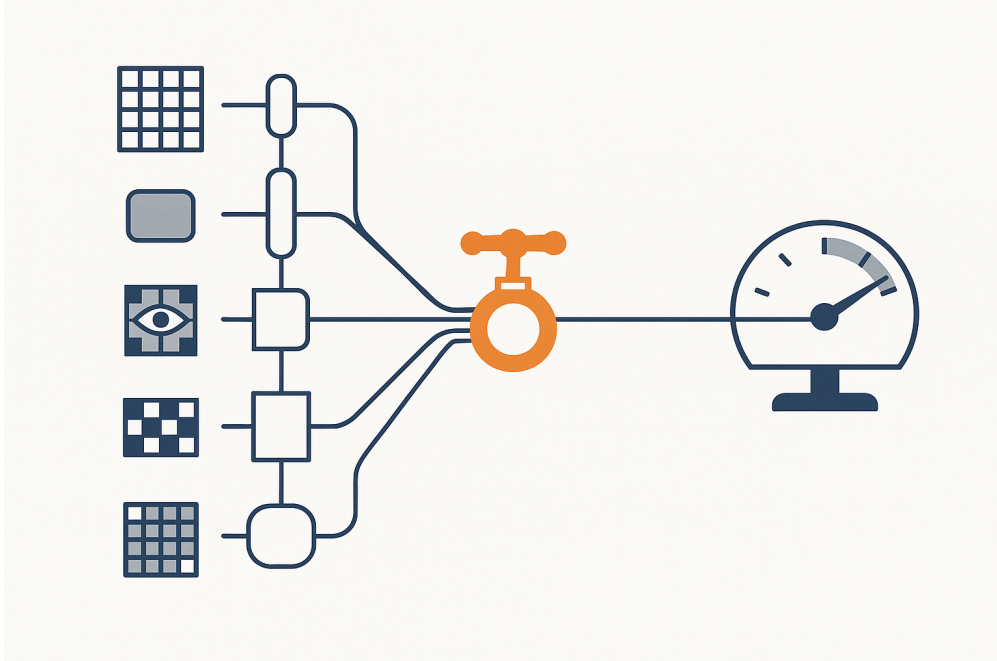
Figure 1: Five architecturally distinct model families are usually assumed to each require their own stability budget. This paper’s central finding is that, under Lagrangian-dual constrained continual learning, the budget is instead set almost entirely by a shared control mechanism, the dual-ascent optimizer’s own schedule, common to every architecture trained with it.
