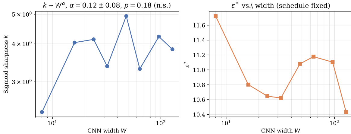
Figure 7: Left: sigmoid sharpness k vs. CNN width on log-log axes; the fitted power law is not statistically significant. Right: \varepsilon^* vs. width for the same family, schedule fixed; consistent with the narrow band reported in Section 6.
