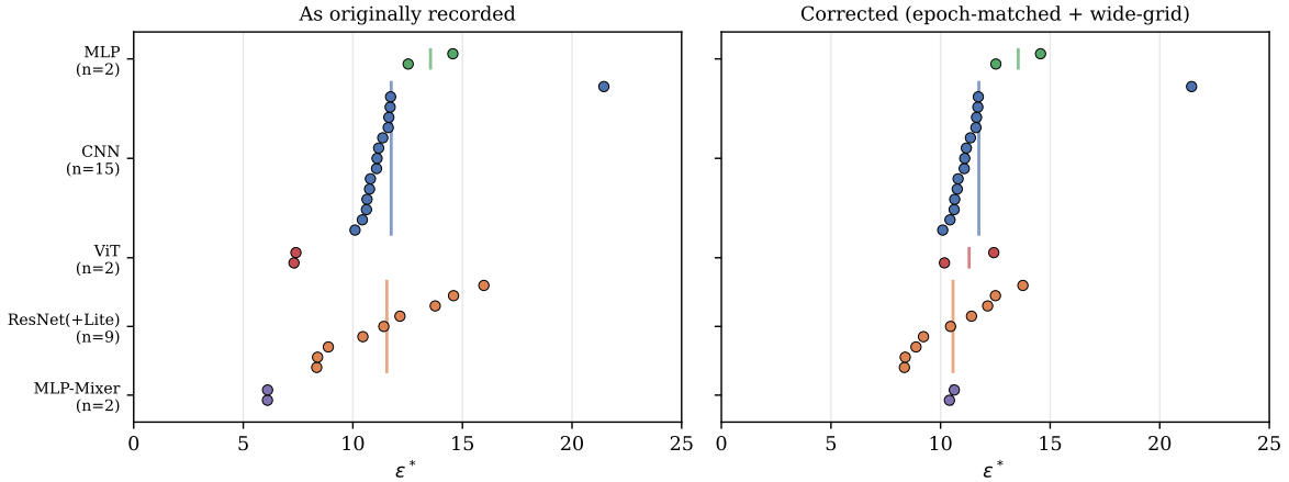
Figure 6: \varepsilon^* by architecture and family, as originally recorded (left) versus corrected (right); vertical bars mark family means. ViT and MLP-Mixer move from a visually distinct low cluster into the same band as the rest of the zoo; CNN and MLP are unchanged. CNN_W8_NoBN (isolated point in the CNN row) remains an outlier in both panels.
