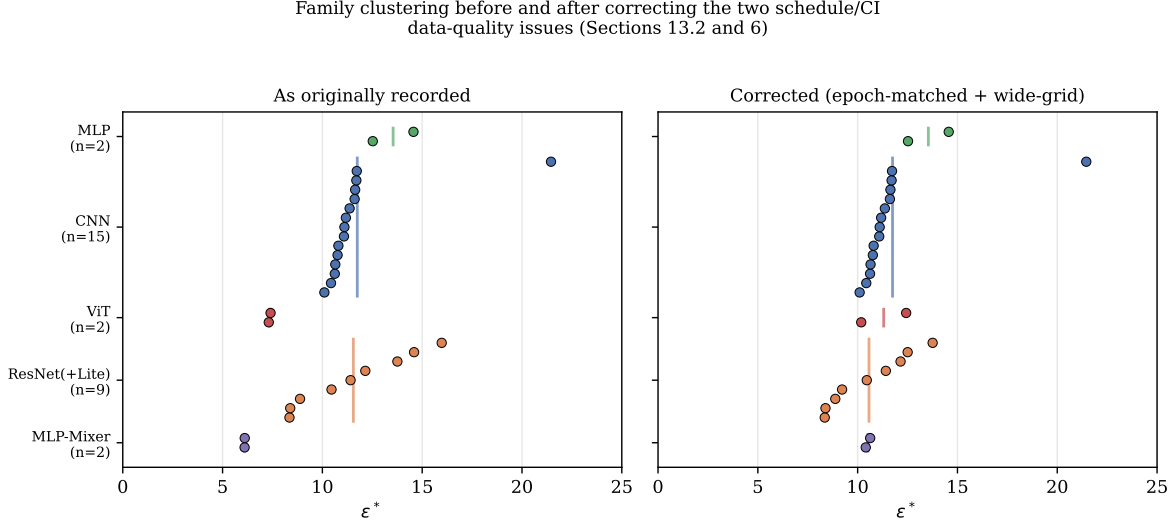
Figure 6: \varepsilon^* by architecture and family, as originally recorded (left) versus corrected (right); vertical bars mark family means. ViT and MLP-Mixer move from a visually distinct low cluster into the same band as the rest of the zoo; CNN and MLP are unchanged. CNN_W8_NoBN (isolated point in the CNN row) remains an outlier in both panels.
