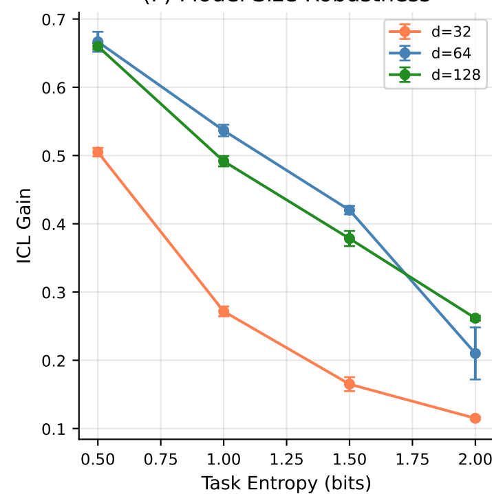
(F) Model Size Robustness
