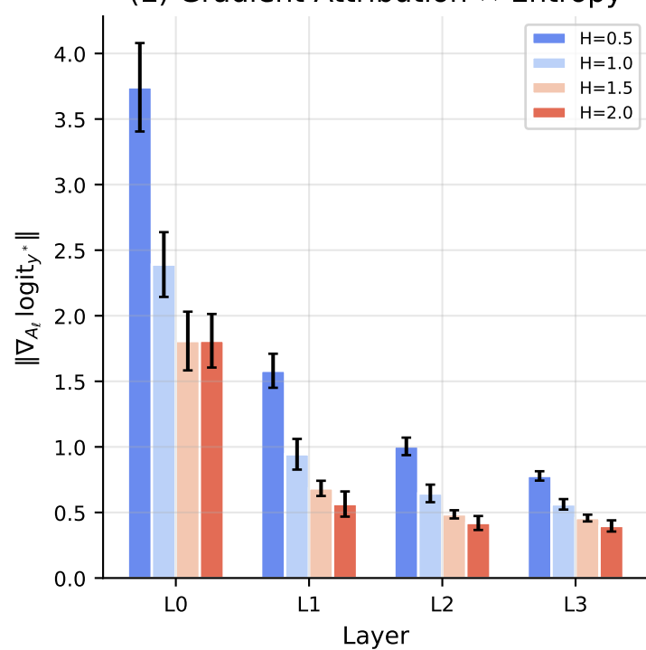
(E) Gradient Attribution \times Entropy
