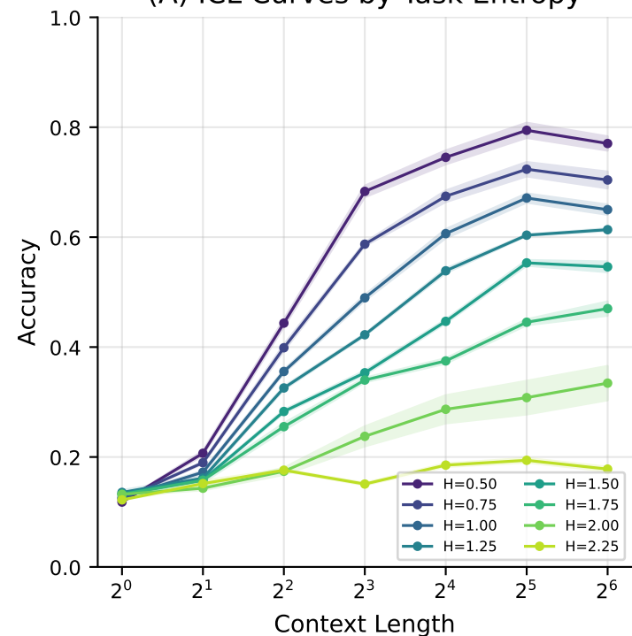
(A) ICL Curves by Task Entropy
