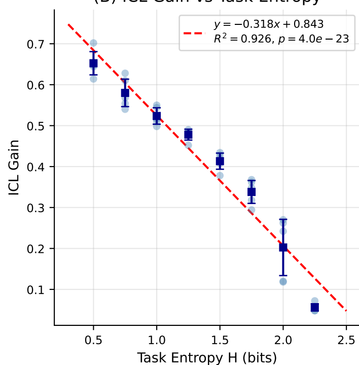
(B) ICL Gain vs Task Entropy
