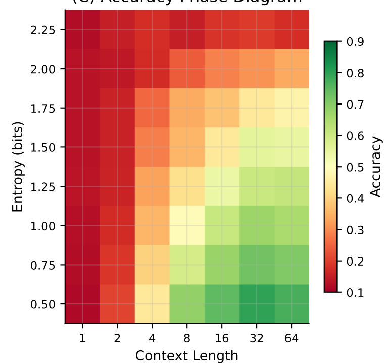
(C) Accuracy Phase Diagram
