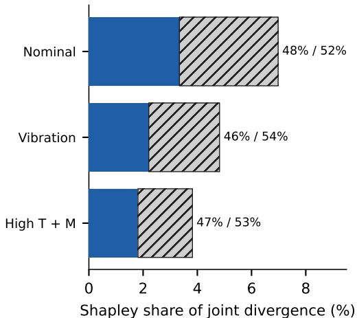
(b) Exact attribution
