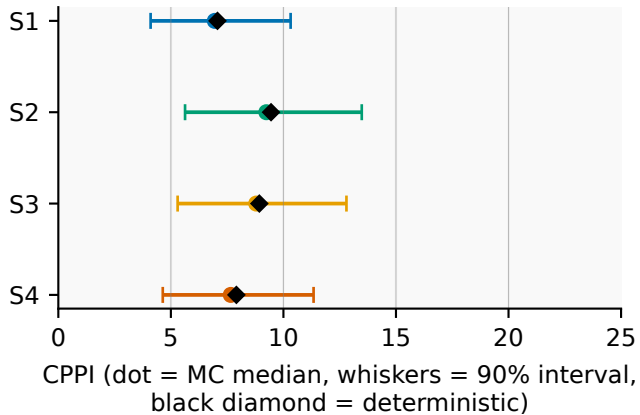
(a) CPPI scores and uncertainty
