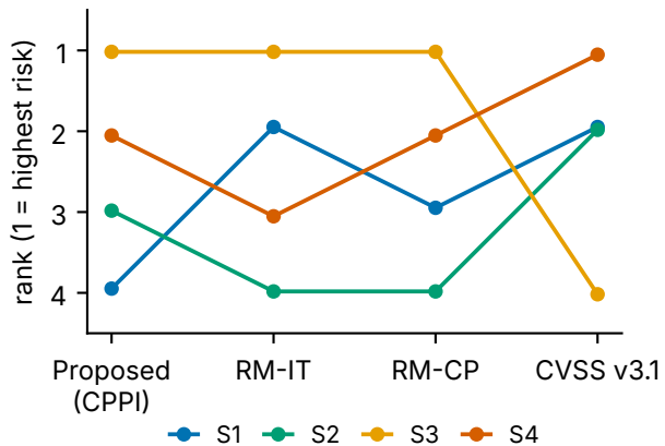
(b) Rank agreement across methods
