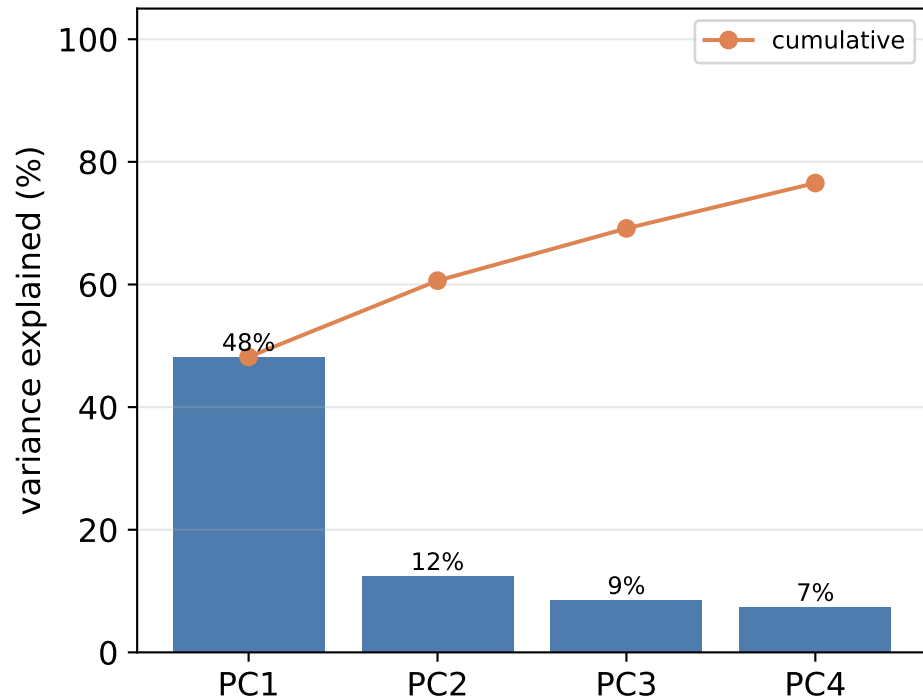
Explained variance (4 qubits = 77%)
