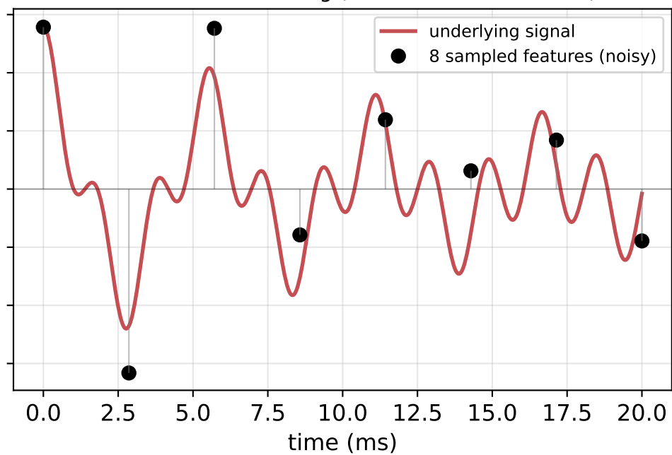
Class 1 — Fault bearing (180 Hz + 3rd harmonic)
