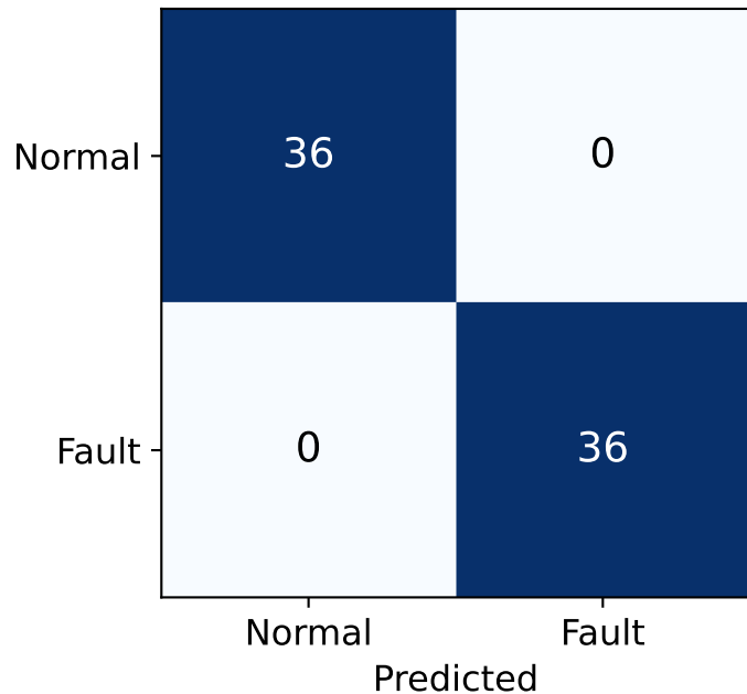
Classical SVM-RBF
