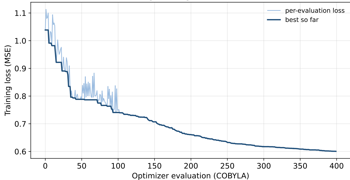
VQC Training Convergence (ideal simulator)
