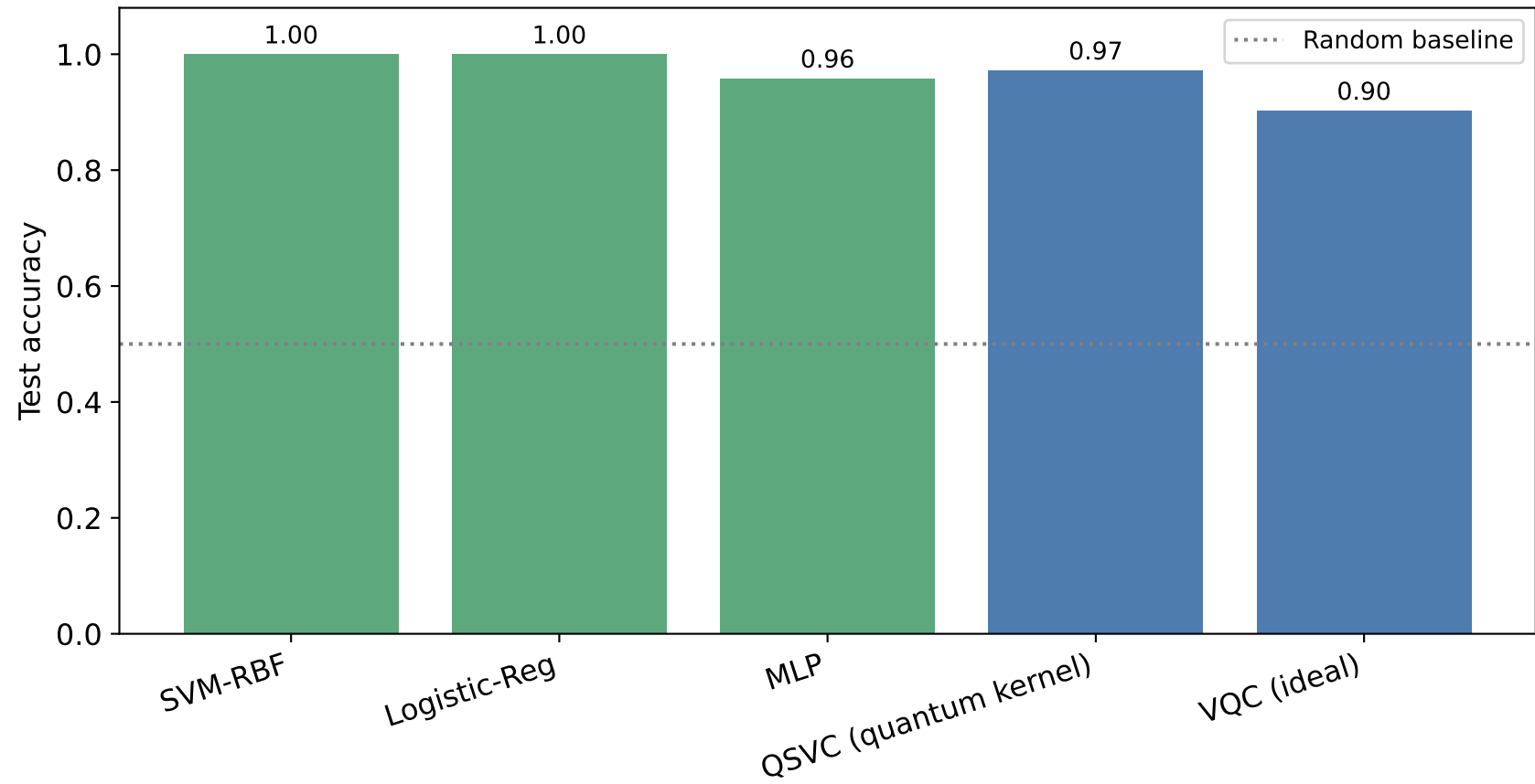
Sensor Fault Classification: Classical vs Quantum Models
